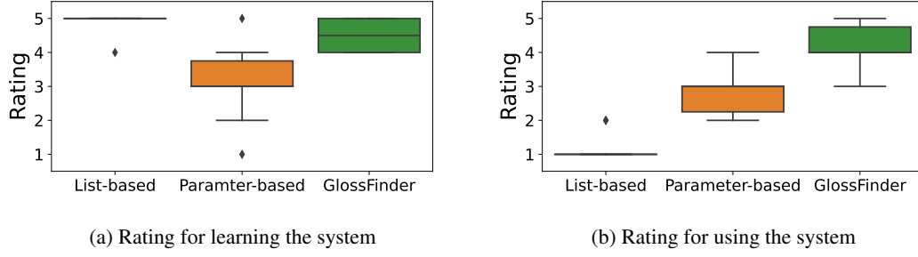
Figure 4: Ratings our participants gave to the benchmark systems during the trials. The rating for learning the system was collected both before and after the trial to cope with the bias from the system introduction and long-term effects of the user getting familiar with the system.
