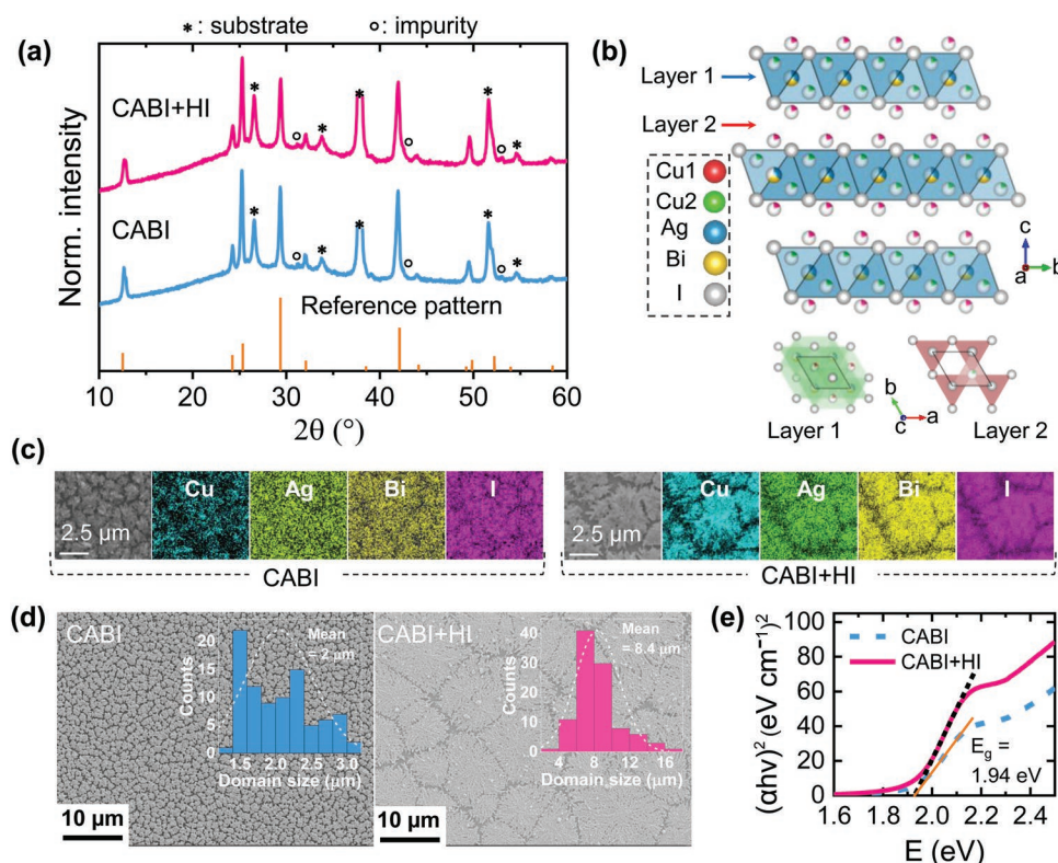
Figure 1. a) XRD patterns of CABI and CABI+HI films deposited on FTO along with the reference pattern of CABI. The highest intense peaks at 25.5°, 29.5° and 42.2° correspond to (012), (104) and (110) crystal planes, respectively. The peaks marked with the asterisk and open circle symbols denote the XRD reflections corresponding to the FTO substrate and impurities, respectively. The substrate's peak at 37.8° is not shown completely. b) Crystal structure of CABI. c) EDS maps of CABI and CABI+HI films showing the distribution of the elements. d) SEM images of CABI and CABI+HI films. Insets are the size distribution of CABI domains in the films. e) Tauc plots of CABI and CABI+HI films.
