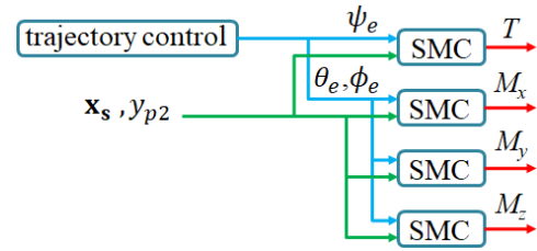
FIGURE 5. The angular position control structure.
