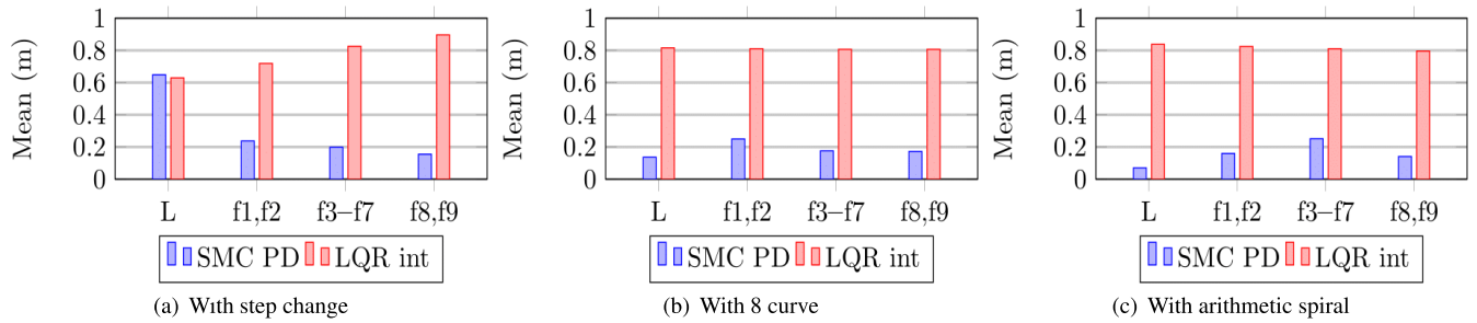
FIGURE 8. Mean value of Euclidean distance from setpoints for the two different control designs.
