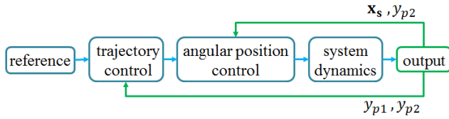
FIGURE 3. Block diagram of SMC PD control design.
