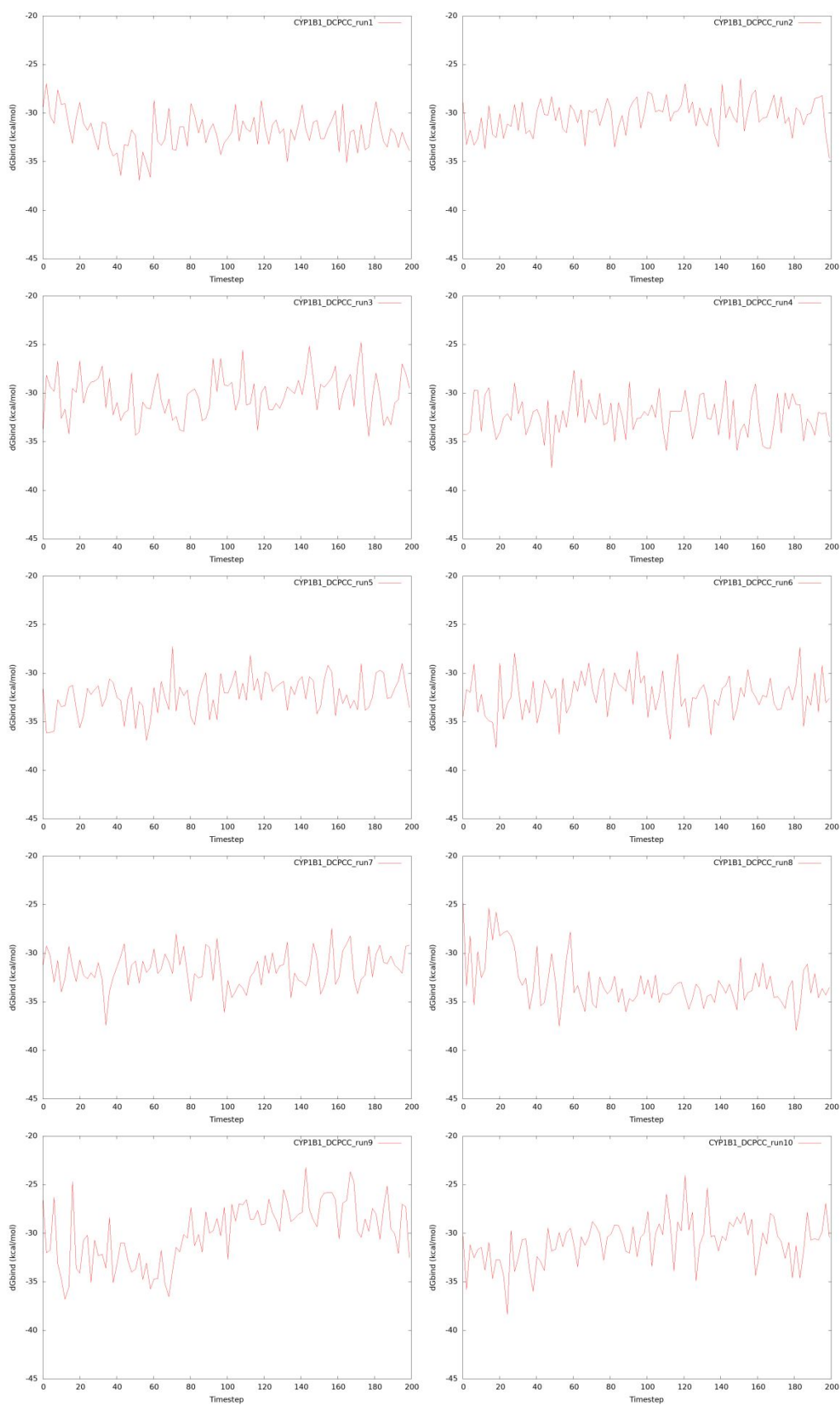
Figure S4. \Delta G_{\text{bind}} of DCPCC-CYP1B1 complexes. Evolution of \Delta G_{\text{bind}} of all DCPCC-CYP1B1 complexes during the simulations (runs 1-10) is shown.
