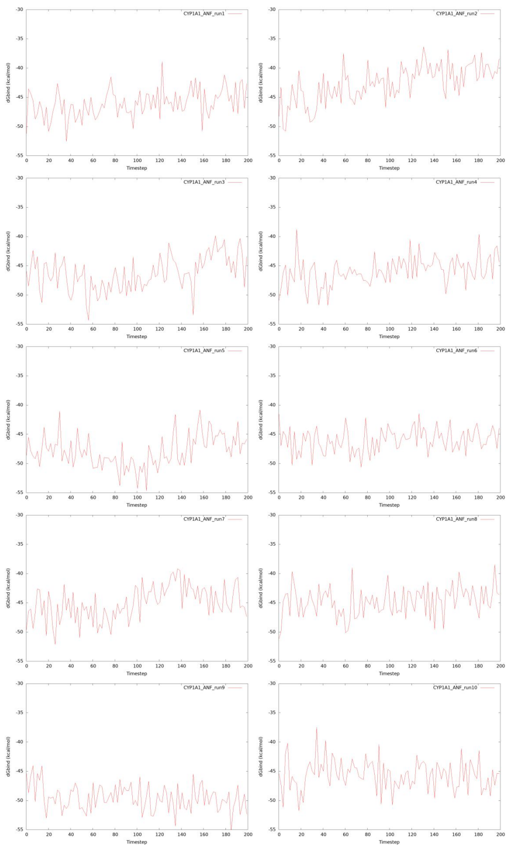
Figure S6. DG_{\text{bind}} of ANF-CYP1A1 complexes. Evolution of DG_{\text{bind}} of all ANF-CYP1A1 complexes during the simulations (runs 1-10) is shown.
