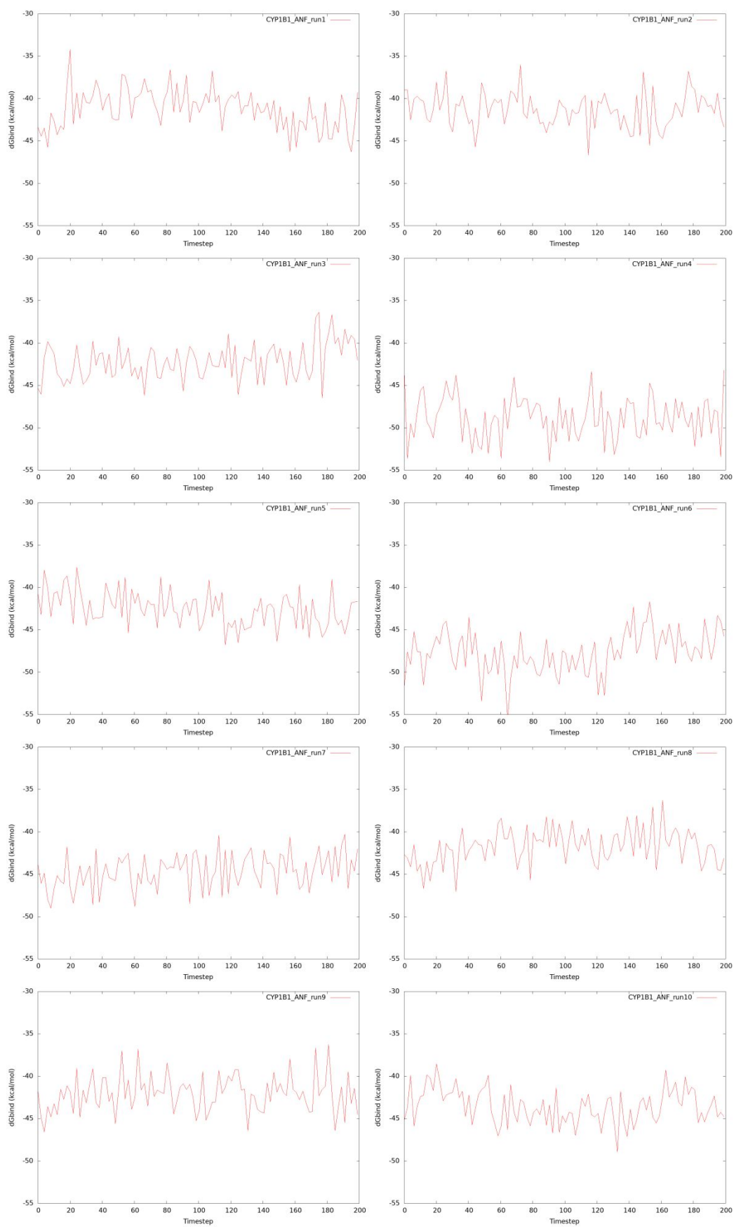
Figure S8. DG_{bind} of ANF-CYP1B1 complexes. Evolution of DG_{bind} of all ANF-CYP1B1 complexes during the simulations (runs 1-10) is shown.
