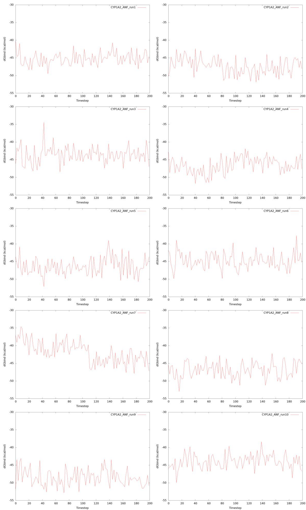
Figure S7. DG_{\text{bind}} of ANF-CYP1A2 complexes. Evolution of DG_{\text{bind}} of all ANF-CYP1A2 complexes during the simulations (runs 1-10) is shown.
