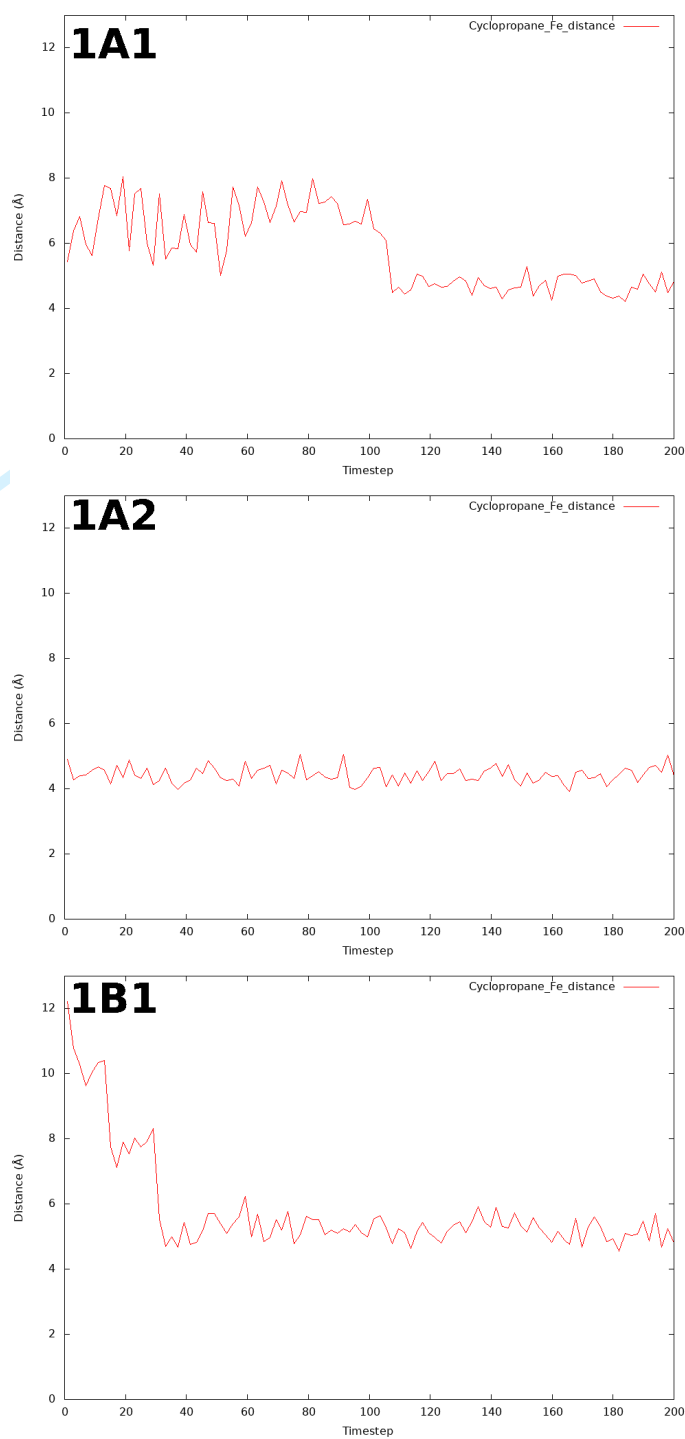
Figure S5. Distance between DCPCC cyclopropane and heme Fe during the simulations. Graphs for the complexes with the lowest DG_{total} are shown (run 2 for 1A1, run 5 for 1A2 and run 8 for 1B1).
