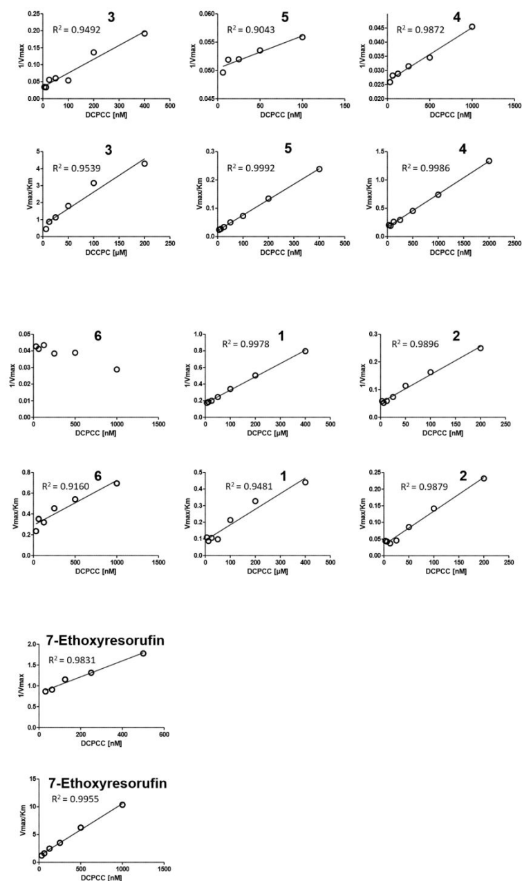
Figure S1. The effect of DCPCC concentration on apparent constants of 1/V_{max} and V_{max}/K_m of probe oxidation reactions of different coumarin derivatives (1- 6) and 7-ethoxyresorufin. Incubation mixture contained 0–40 \mu M of the indicated substrate, 2.5 nM CYP1A2 enzyme, 20% NADPH regenerating system and 0–1 \mu M DCPCC in 100 mM Tris-HCl pH 7.4. 100% reaction did not contain inhibitor, and blank samples did not contain CYP1. The data at 5 - 7 DCPCC concentration was analyzed with Michaelis-Menten equation v = S * V_{max} / (K_m + S) , in which v is the reaction rate, S substrate concentration, V_{max} is the apparent V_{max} -value and K_m the apparent K_m -value at each DCPCC concentration.
