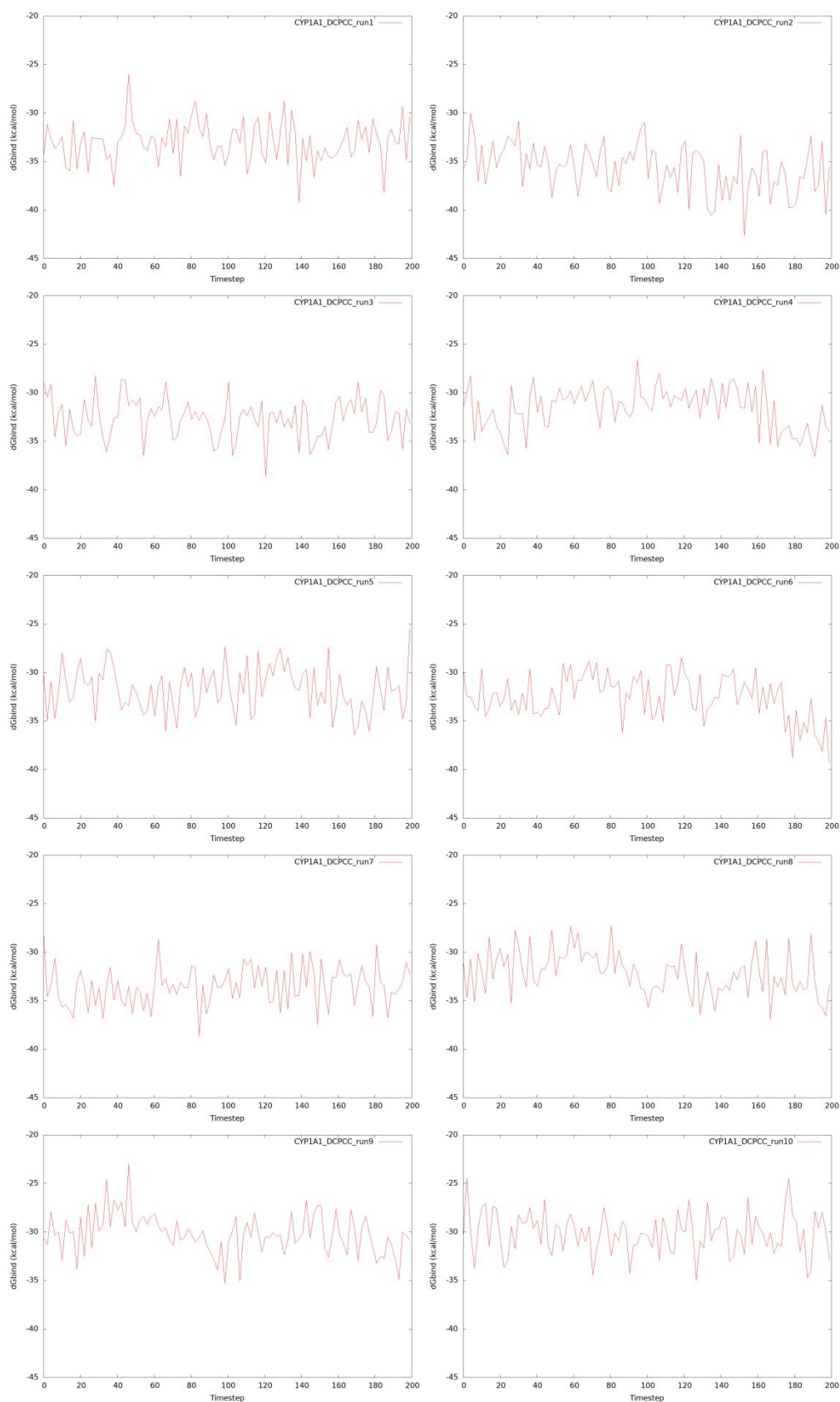
Figure S2. DG_{\text{bind}} of DCPCC-CYP1A1 complexes. Evolution of DG_{\text{bind}} of all DCPCC-CYP1A1 complexes during the simulations (runs 1-10) is shown.
