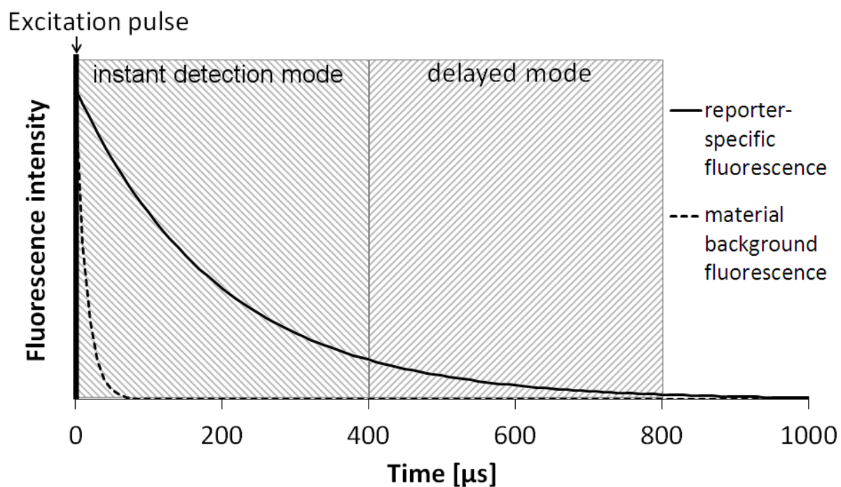
Fig. 2. Illustration of the modes used for time-resolved measurement of Eu(III)-nanoparticles. Non-delayed measurement at 0-400 \mu\text{s} includes also short-lived background fluorescence (dashed line). In the delayed measurement window only long-lived fluorescence originating from the reporters (solid line) can be measured.
