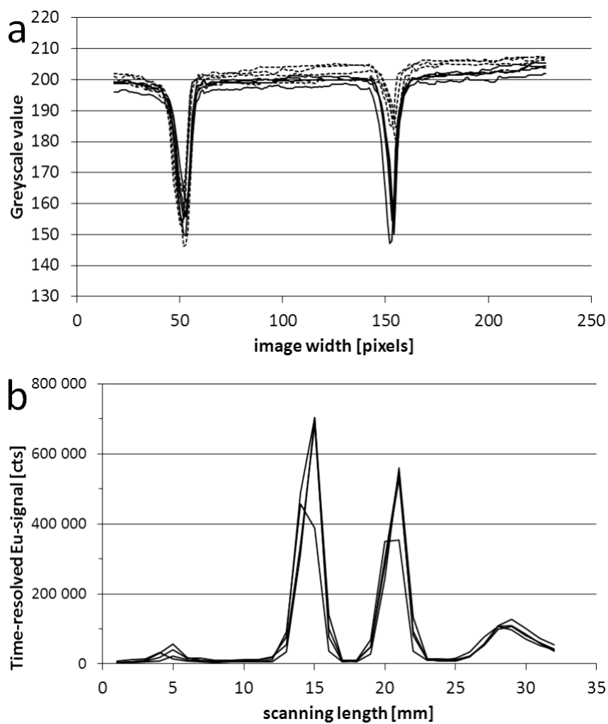
Fig. 5. Examples of signal profiles of PSA with a) reflectometric measurement of colloidal gold and b) delayed time-resolved fluorescence scanning of Eu(III)-nanoparticles. Reactions with maximal signal (100 ng/ml PSA) are depicted with solid line and reactions containing no analyte are with dashed line. Both reactions are presented with four replicates.
