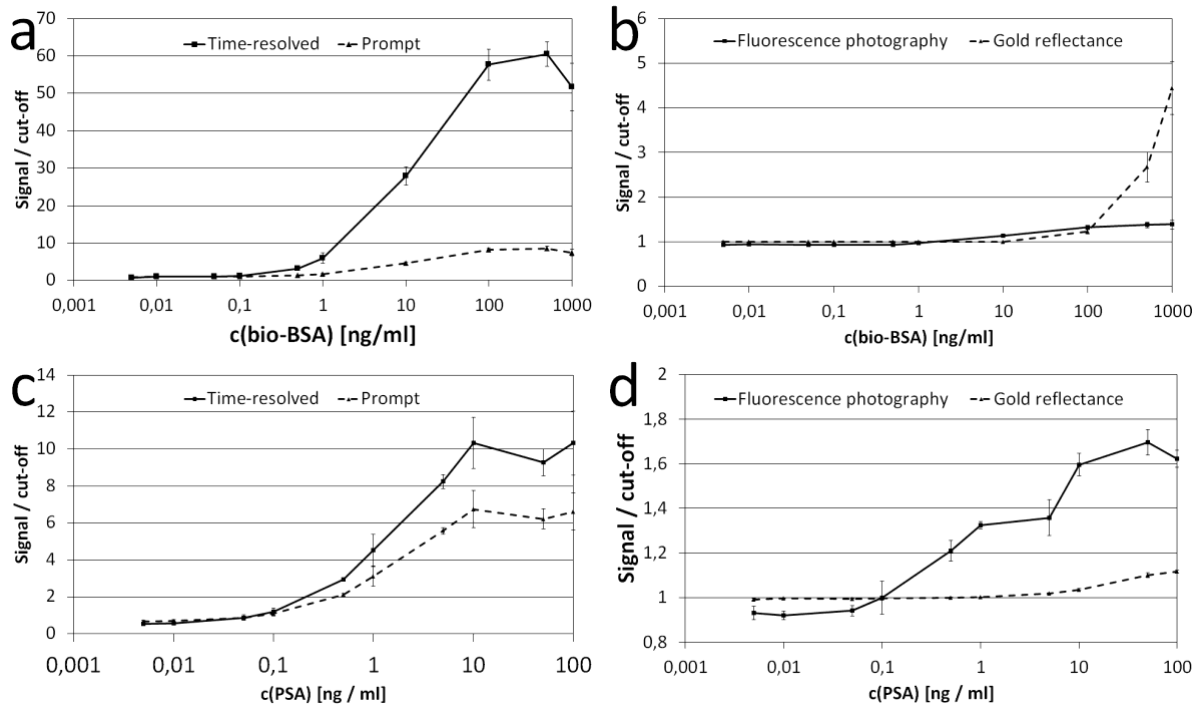
Fig. 4. Dose-response graphs of PSA and bio-BSA in their respective assays. In graphs a) and c) assays with scanning-based detection systems and in graphs. Delayed time-resolved measurement with solid and short-lived measurement are drawn with dashed line. In graphs b) and d) imaging-based detection systems. Standard deviations in both directions depicted as error bars. Limit of detection marked with x in each curve.
