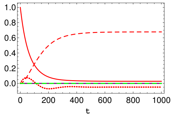
FIG. 2. (Color online) Mean value of different two-qubit observables as a function of time, when the evolution starts in the state |11\rangle_f and we use the master equation (25) in partial secular approximation. As defined in the main text, we plot P_{11}(t) (solid red), P_{00}(t) (dashed red), C_0(t) (dotted red), C_1(t) (dashed green), C_2(t) (solid purple). C_1 and C_2 remain null during the evolution, while using the master equation in partial secular approximation C_0 varies and stabilizes to a non-zero value after the thermalization time, showing the appearance of steady-state coherences. On the contrary, the full secular approximation would keep C_0 null as well.
