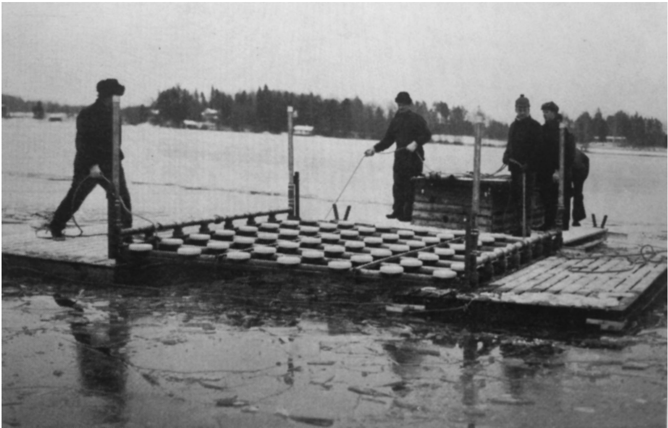
Fig. 3 Nokia aerators being immersed in Tuusulanjärvi in 1972. Originally published in Nokia (1972b, p. 29), photographer unknown, reproduced with the permission of Nokia Ltd
