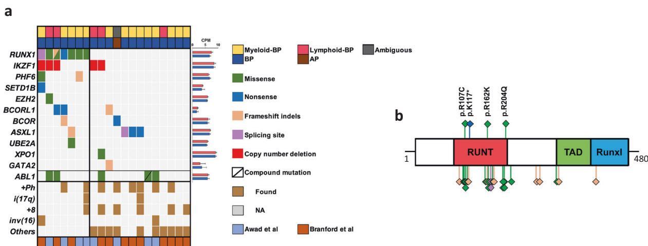
Fig. 1 Spectrum of RUNX1 mutations in BP-CML patients. a Landscape of somatic mutations identified by WES in BP-CML samples from our cohort ( n = 8 , 4 RUNX1 mut and 4 RUNX1 wt ) and from Branford et al. [24] ( n = 12 , 3 RUNX1 mut and 9 RUNX1 wt ). Complete lists of identified mutations are detailed in Supplementary Table 4. Explanatory tracks from top to bottom show phenotype of the blast (myeloid-BP, lymphoid-BP, and Ambiguous) and phase of CML (accelerated phase AP or blast phase BP) cases. The filling color indicates the type of the variant. The average expression of the genes in 4 RUNX1 mut (red) and 5 RUNX1 wt (blue) BP-CML samples is shown on the right expressed as counts per million mapped reads (CPMs). Bar lengths indicate means and errors. Chromosomal
