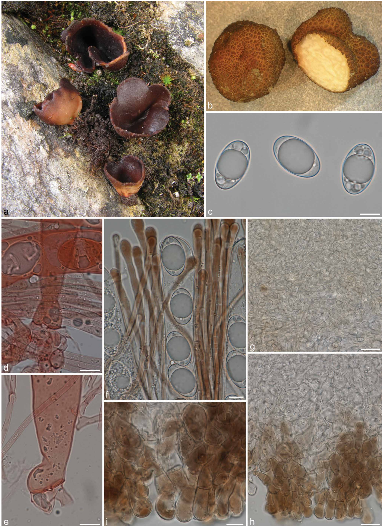
Fig. 3 Balsamia . a. Balsamia aestivalis apothecia; b. Balsamia platyspora ascomata; c–h. Balsamia aestivalis : c. ascospores; d–e. ascus base showing crozier (in CR); f. asci and paraphyses with reddish brown content; g. medullary excipulum of textura intricata (in KOH); h. outer excipulum of textura angularis , outermost cells elongated, forming short, hyphoid, fasciculate hairs with evenly brown content (in KOH); i. outermost hyphoid hairs (in water), end cell slightly club-shaped with a thin gelatinous or amorphous sheath (a, c–f: KH.10.133; b: TUR206101; g–i: KH.10.117). — Scale bars: c–f, i = 10 \mu m, g–h = 20 \mu m; a–c, f living material; d–e, g–i from dried material. — Photos: a, c–i K. Hansen; b S. Huhtinen.
