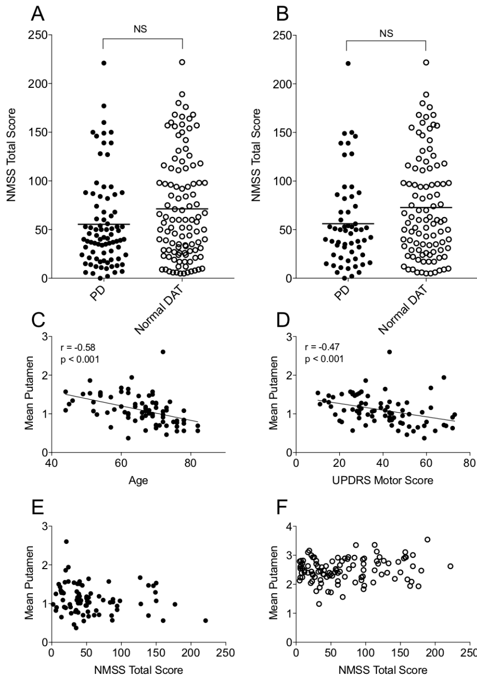
Figure 1. A. NMSS total score in PD patients and normal DAT patients. B. NMSS total score in patients with no dopaminergic medication. Relationship between mean putamen SBR and C. age in PD patients, D. MDS-UPDRS motor score in PD patients, E. NMSS total score in PD patients and F. NMSS total score in normal DAT patients. DAT = dopamine transporter, NMSS = Non-motor symptoms scale, NS = Not significant, MDS-UPDRS = the Movement Disorder Society Unified Parkinson's Disease Rating Scale, PD = Parkinson's disease.
