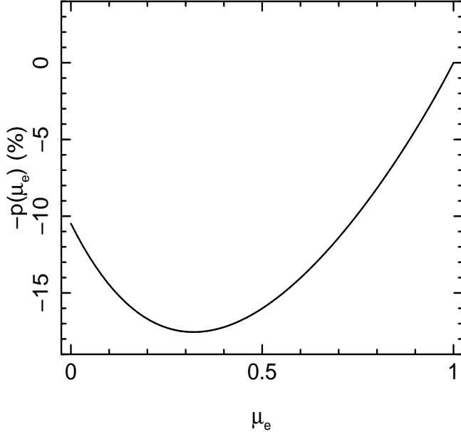
Figure 4. Polarization degree as a function of emission angle assumed for this Paper. We use the analytic function p(\mu_e) = 50\%(1 - \mu_e) - 23\%[\exp\{(1 - \mu_e)^{1.6}\} - 1] , designed to mimic the results of ST85 for the \tau_0 = 1 case. This Figure can be compared with Figure 5 of ST85.
