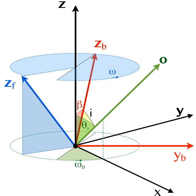
Figure 1. Coordinate system used in this Paper. We define right handed Cartesian coordinate systems with z-axes aligned with the BH, flow and binary spin axes. The BH (black) and binary (red) z-axes are misaligned by the angle \beta and the binary system x-axis is chosen to be in the unique plane shared by the BH and binary z-axes. The vector \hat{o} represents the observer’s line of sight, and the BH x-axis is chosen as the projection of this vector onto the BH equatorial plane. The flow z-axis (blue) precesses around the BH z-axis with precession angle \omega , always maintaining the misalignment angle \beta . The flow and binary z-axes are therefore aligned when \omega = 180^\circ and misaligned by an angle 2\beta when \omega = 0^\circ .
