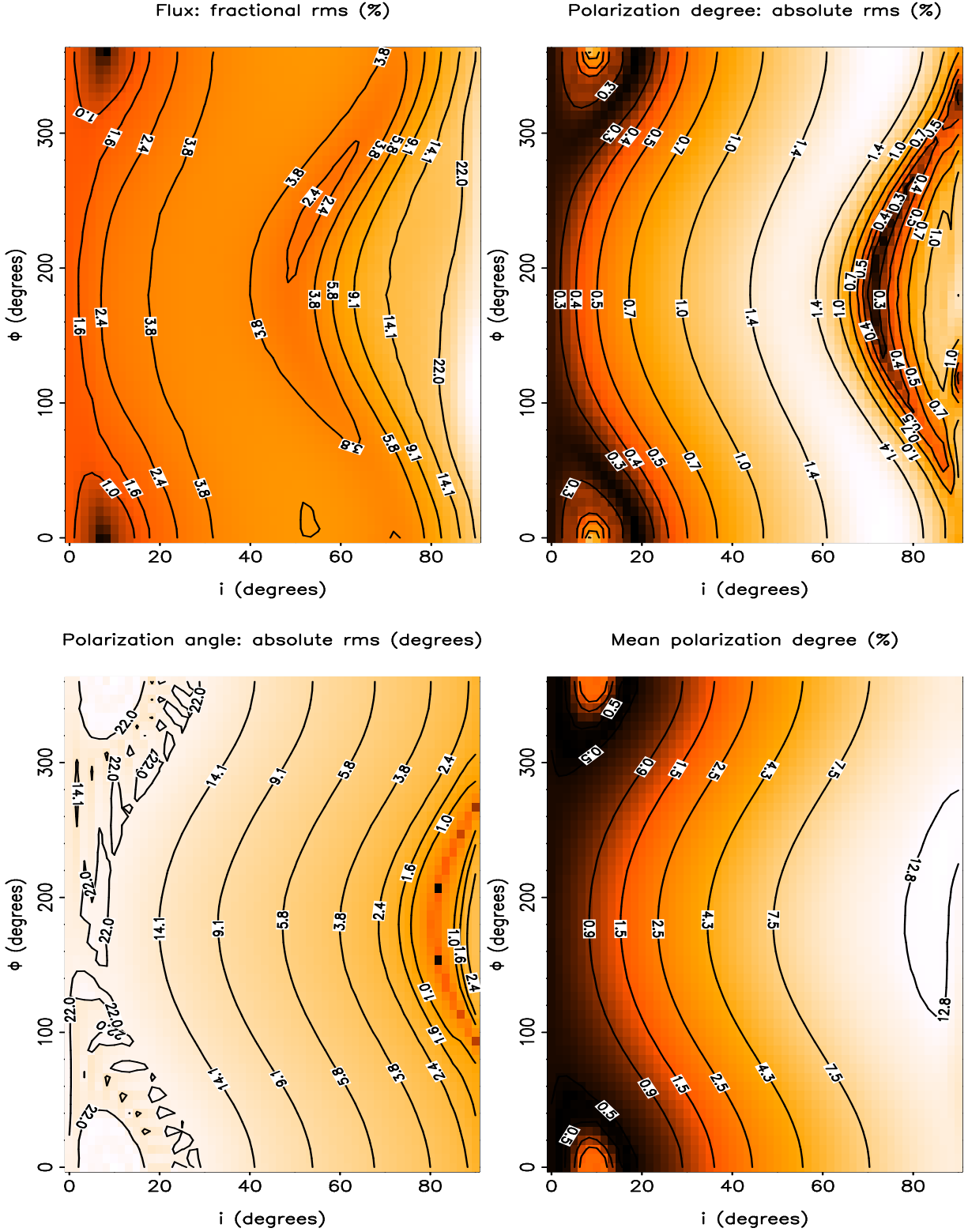
Figure 9. Top-Left: Fractional rms in the first harmonic of the flux modulation plotted as a function of the two viewing angles, i and \Phi , with contours labelled as percentages. Top-Right: Absolute rms in the first harmonic of the polarization degree modulation, with contours again labelled as percentages. Bottom-Right: Mean polarization degree, with contours once again labelled as percentages. Bottom-Left: Absolute rms in the first harmonic of the polarization angle modulation, with contours now labelled in degrees. The colors in each plot follow separate logarithmic scales. We see that the amplitude of the flux and polarization degree modulations increase with inclination angle, i , whereas the amplitude of the polarization angle modulation reduces with i . Note the slight asymmetry in all plots around \Phi = 180^\circ , which occurs because a \neq 0 .
