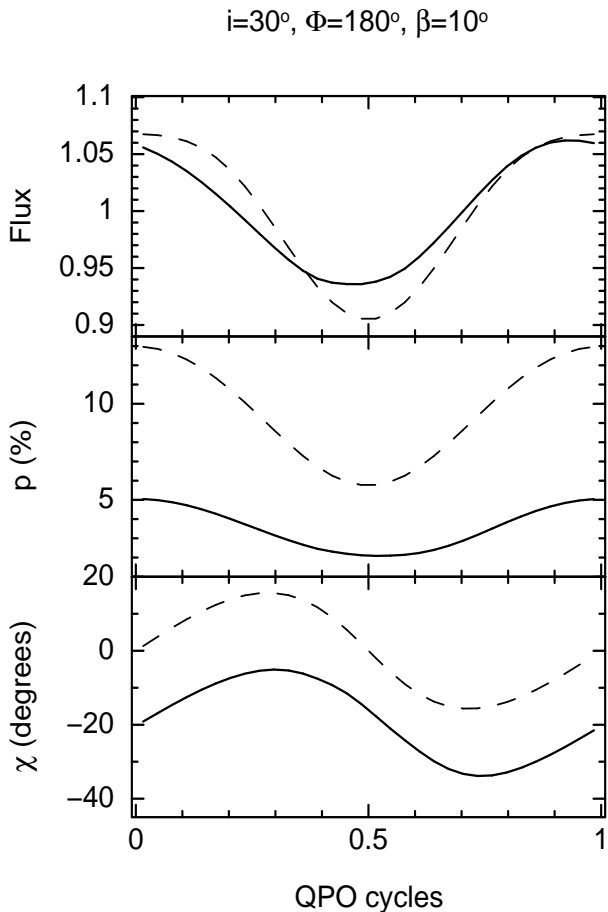
Figure 7. Flux, polarization degree and polarization angle plotted against QPO phase for the low inclination model. Solid and dashed lines again refer to the fully relativistic model and the Newtonian comparison respectively. The fractional rms (for the full model) in the first and second harmonics respectively is 4.6% and 0.25% for the flux. The absolute rms in the first and second harmonics is respectively 1.1% and 0.05% for the polarization degree and respectively 10.0^\circ and 1.0^\circ for the polarization angle.
