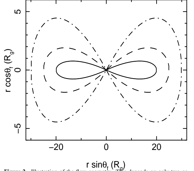
Figure 2. Illustration of the flow geometry. This depends on only two parameters: the scale height h/r and the outer radius in units of R_g , r_o . For r \ll r_o , this function has a constant opening angle, but curves around into a tear drop shape for larger r . We show three example parameter combinations: h/r = 0.1 , r_o = 20 (solid line), h/r = 0.2 , r_o = 25 (dashed line) and h/r = 0.4 , r_o = 30 (dot-dashed line). In this Paper, we consider the first of these geometries, represented by the solid line.
