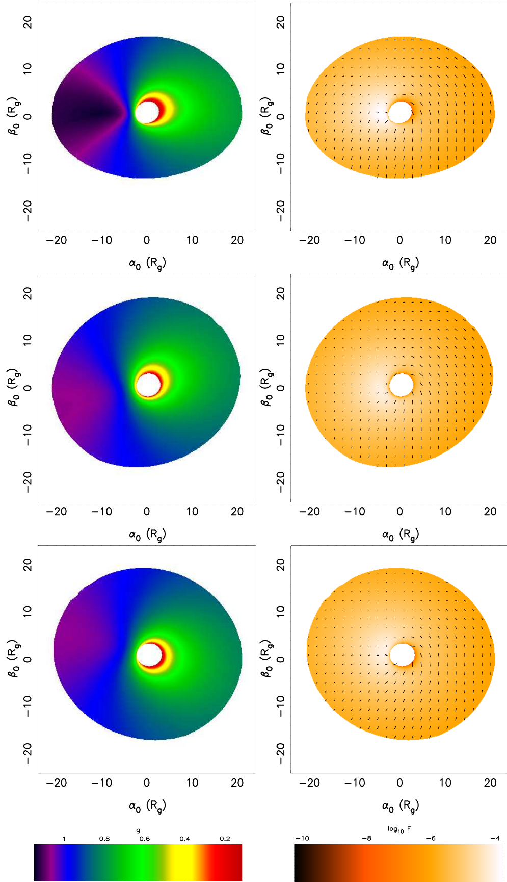
Figure 8. Images of the flow for three precession angles for the model with i = 30^\circ , \Phi = 180^\circ , \beta = 10^\circ and h/r = 0.1 . The left hand side pictures blueshift and the right hand side pictures flux with the polarization vector overlaid, normalised to the maximum observed polarization degree. The three precession angles, in units of cycles, are \omega = 0, 0.3125 and 0.625 from top to bottom respectively. Full movies corresponding to these images can be found at http://figshare.com/articles/Polarization_modulation_gifs/1351920 . Individual movies can alternatively be found on YouTube: www.youtube.com/watch?v=TS-e-iXofu8&feature=youtu.be (blueshift) and www.youtube.com/watch?v=GjIRfkor_s&feature=youtu.be (flux and polarization).
