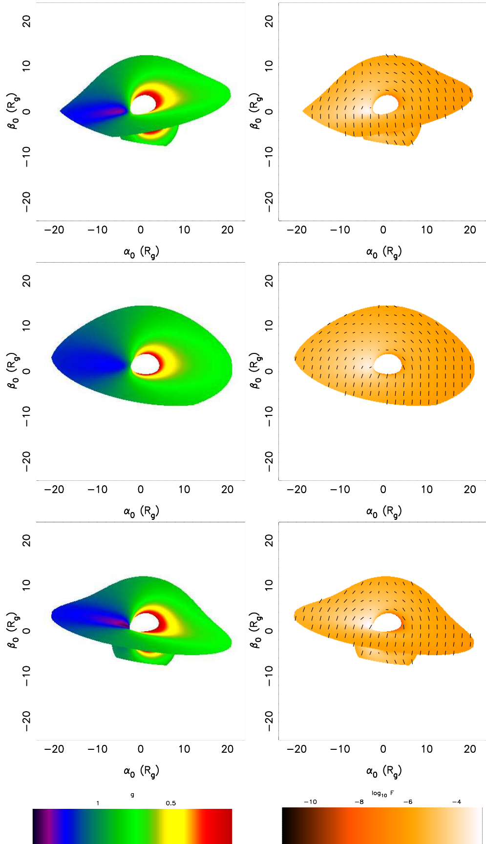
Figure 5. Images of the flow for three precession angles for the model with i = 70^\circ , \Phi = 110^\circ , \beta = 10^\circ and h/r = 0.1 . The left hand side pictures blueshift and the right hand side pictures flux with the polarization vector overlaid, normalised to the maximum observed polarization degree. The three precession angles pictured, in units of cycles, are \omega = 0, 0.3125 and 0.625 from top to bottom respectively. The full movies for these images can be found at http://figshare.com/articles/Polarization_modulation_gifs/1351920 . Individual movies can alternatively be found on YouTube: www.youtube.com/watch?v=Q2CwOGKVC9U&feature=youtu.be (blueshift) and www.youtube.com/watch?v=E3kYAnS3pQI&feature=youtu.be (flux and polarization).
