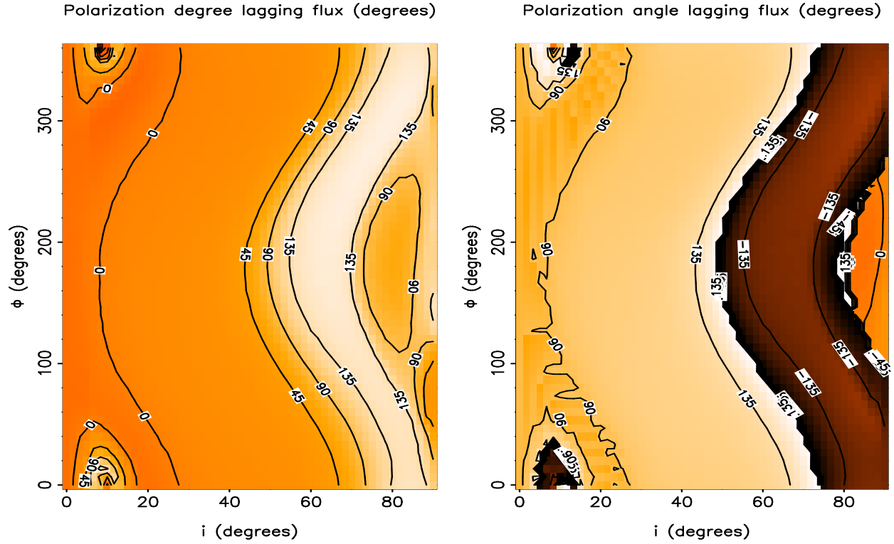
Figure 10. Left: Phase lag in degrees between the polarization degree and the flux, with positive lag meaning that p lags F . Here, we only plot for the fundamental and color scales linearly from -180^\circ (darkest) to 180^\circ (lightest). We see that the model predicts the oscillation in polarization degree to lag the first harmonic of flux for almost the full range of viewing angles. Right: Phase lag between polarization angle and flux. The model predicts the magnitude of the phase lag between \chi and F to be large for most of parameter space.
