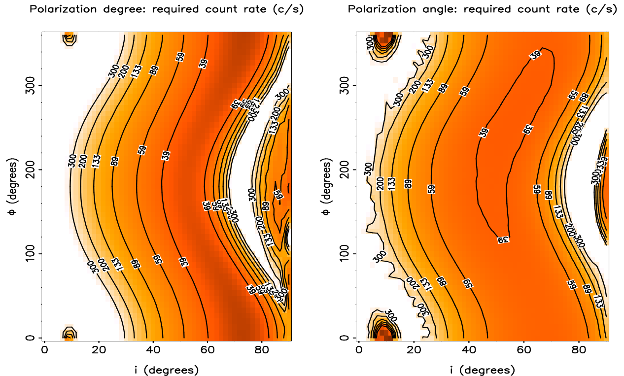
Figure 11. Required count rate in order to detect a modulation in polarization degree (left) and angle (right). We assume a 200 ks exposure and a modulation factor of \mu = 0.5 . See text for more details.
