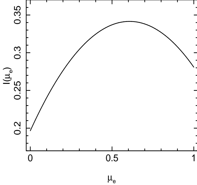
Figure 3. Intensity as a function of emission angle assumed for this Paper. We use the analytic function I(\mu_e) \propto 1 + 1.1(1 - \mu_e) - 1.4(1 - \mu_e)^2 , designed to mimic the results of ST85 for the \tau = 1 case. This Figure can be compared with Figure 4 of ST85, except we use a different normalization.
