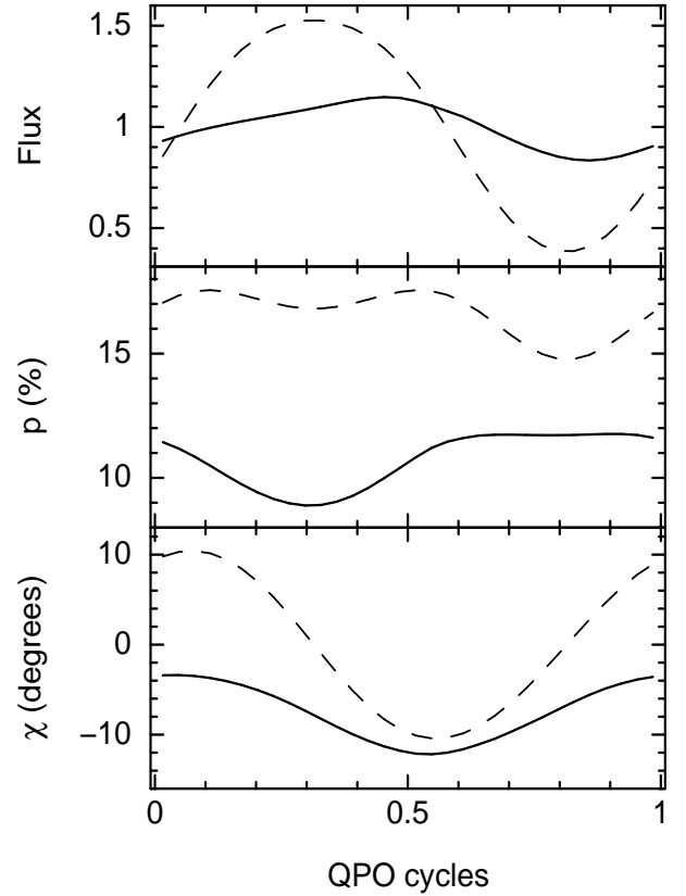
Figure 6. Flux, polarization degree and polarization angle plotted against QPO phase for the high inclination model. The solid lines are for the fully relativistic model and dashed lines representing a simple Newtonian approximation are included for comparison. The fractional rms (for the full model) in the first and second harmonics respectively is 10.0% and 2.24% for the flux. The absolute rms in the first and second harmonics is respectively 1.0% and 0.3% for the polarization degree and respectively 3.1^\circ and 0.2^\circ for the polarization angle.
