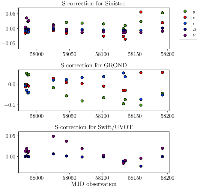
Figure 3. S-correction for LCO+Sinistro (top panel), GROND+2.2m (middle panel) and Swift /UVOT (lower panel). Filled dots are coded as in the label (top right corner).
