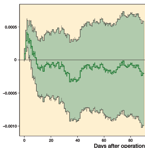
Aalen additive plot with cumulative coefficients (y-axis) with 95% confidence interval comparing cemented with cementless total hip arthroplasties within 90 days of surgery.
