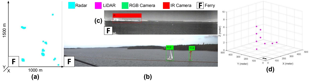
Fig. 2. An example of the output of object detection module in the proposed framework. (a) location intensities of the detected objects by radar; (b) two detected objects (boat and seamark) by RGB camera; (c) one detected object (land) by IR camera and (d) 3D point cloud data for two detected objects (boat and seamark). In the bottom left corner of all figures, 'F' box indicates the location of the ferry.
