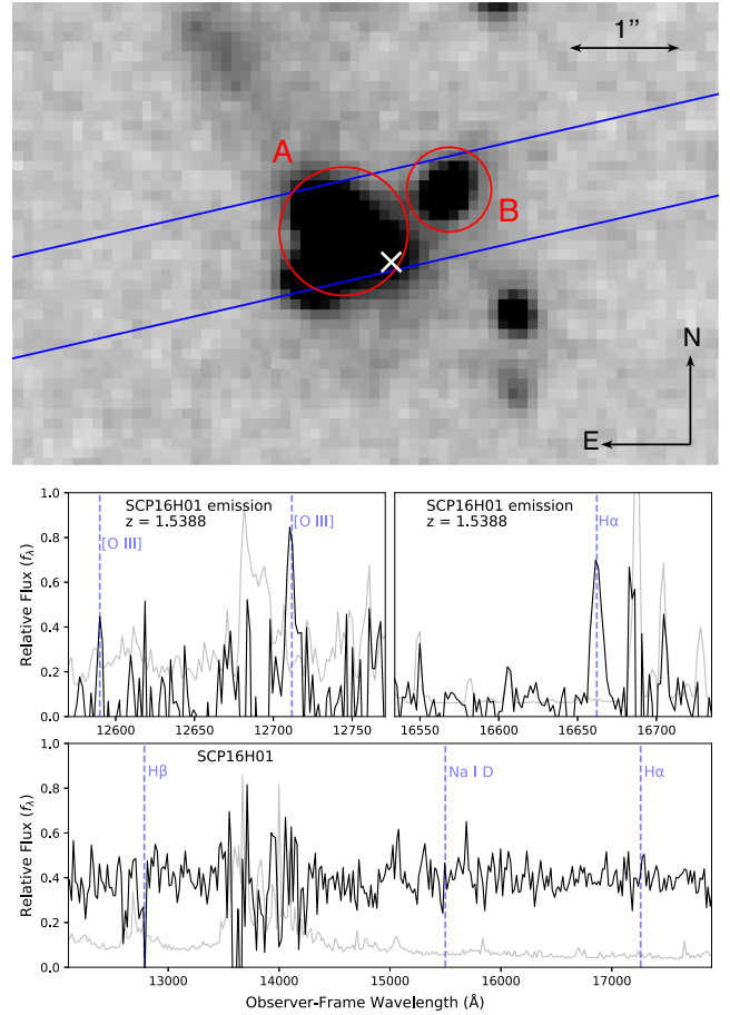
Figure 10. Upper panel: stacked HST WFC3/IR F105W image showing the host structure of SCP16H01. The two components with spectra are indicated in red (see the text), the position of the X-Shooter slit is in blue and the position of SN Ia SCP16H01 is indicated by a white ‘x’. Middle panel: X-Shooter spectrum of Component B of the SCP16H01 host structure, showing H \alpha and [O III] 5007 \text{\AA} emission at z = 1.5388 . Lower panel: X-Shooter spectrum of Component A of the SCP16H01 host structure, showing no secure redshift, with the expected positions of lines placed at the cluster redshift ( z = 1.63 ) indicated for reference. This spectrum is corrected for contamination by Component B. Key as given in Fig. 6.
