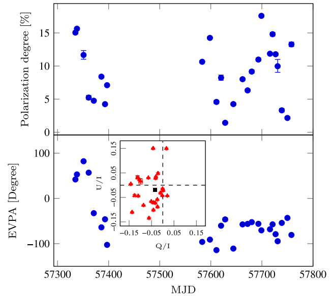
Figure 8. Top panel: degree of polarization in the optical ( R band) obtained with the Nordic Optical Telescope. Bottom panel: same for the polarization angle. The inset shows the source polarization measurements in Q/I-U/I plane. The black square in the Q/I-U/I plane is the mass centre of weighted average of the Q/I and U/I values.
