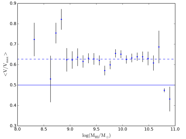
Fig. 5. Mean value \langle V/V_{\text{max}} \rangle binned by HI mass. Error bars are Poisson counting uncertainties. The solid line indicates the value of 0.5 expected for a homogeneous spatial distribution. The dashed line shows the actual average value from the KLUN catalog limited to \log(F_{\text{HI}}) \geq 0.7 .
