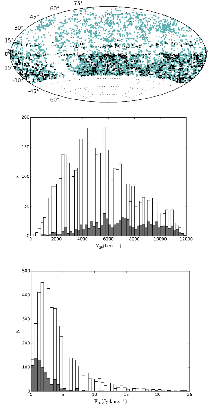
Fig. 1. General statistics of the KLUN HI catalog. Top: Aitoff projection of the KLUN composite Nançay HI-data catalog (cyan dots: Theureau et al. 1998a, 2005, 2007; Paturel et al. 2003b; black dots: the galaxies added in this publication). Middle: distribution of radial velocities (optical convention) for the KLUN composite catalog (white columns) and this paper (gray columns). Bottom: distribution of beam-corrected HI-fluxes (same samples).
