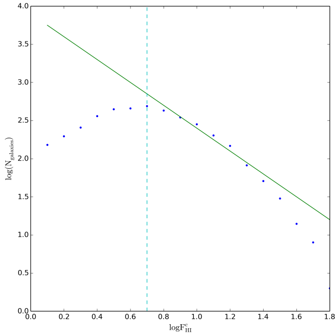
Fig. 4. Logarithmic HI flux distribution. Blue dots are the galaxy counts per 0.1 dex flux bin; the green line shows the expected growth for a pure flux limited sample. The vertical blue dashed line marks the flux limit adopted.
