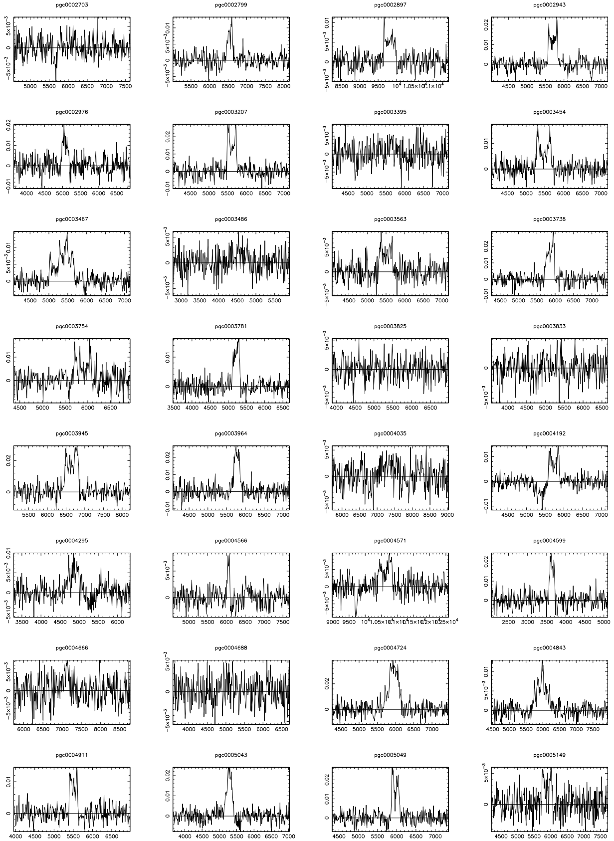
Fig. A.1. 21 cm line profiles of galaxies listed in Table 2 (rest of Fig. 2).
