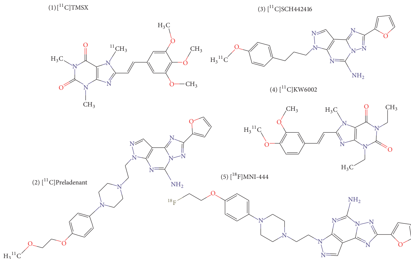
FIGURE 3: Chemical structures of A_{2A} receptor-binding radioligands. ((1) [^{11}\text{C}] TMSX, (2) [^{11}\text{C}] Preladenant, (3) [^{11}\text{C}] SCH442416, (4) [^{11}\text{C}] KW6002, (5) [^{18}\text{F}] MNI-444).
