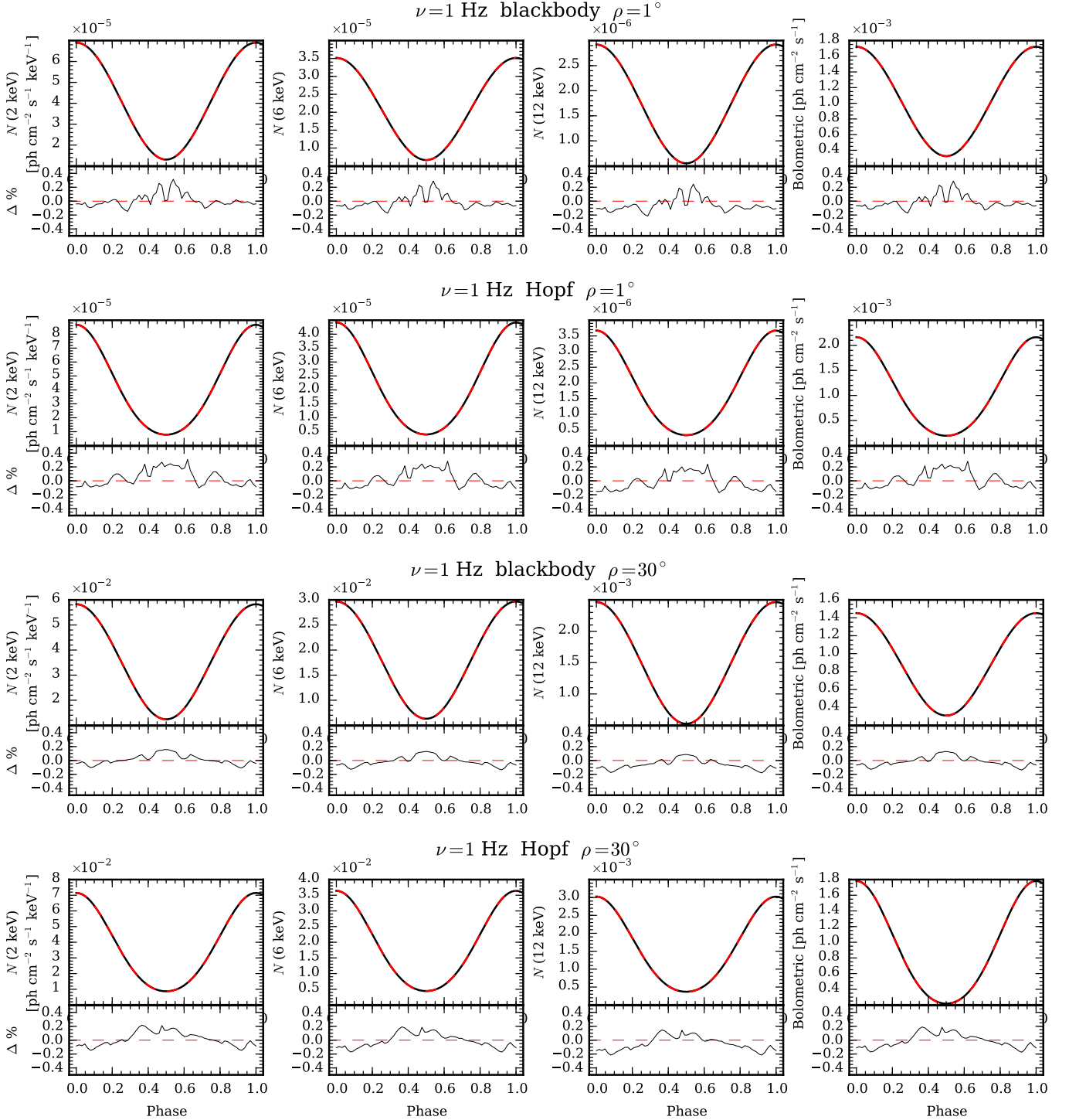
Fig. 8. Light-curve comparisons for Schwarzschild space-time with a slowly rotating spherical star ( R = 12 \text{ km} , M = 1.6 M_{\odot} , \nu = 1 \text{ Hz} , i = 60^{\circ} , \theta_s = 50^{\circ} , \rho = 1^{\circ} , and T_{\text{eff}} = 2 \text{ keV} ) emitting according to a blackbody or Hopf profile with a spot size of either 1 or 30 degrees. The black solid line shows the pulse profiles computed using the S+D approximation (forward-in-time method; see text), and the red dashed line is a profile computed with the code presented here. Lower panel: residuals as \Delta = (\text{model}_{\text{S+D}}/\text{model} - 1) \times 100\% .
