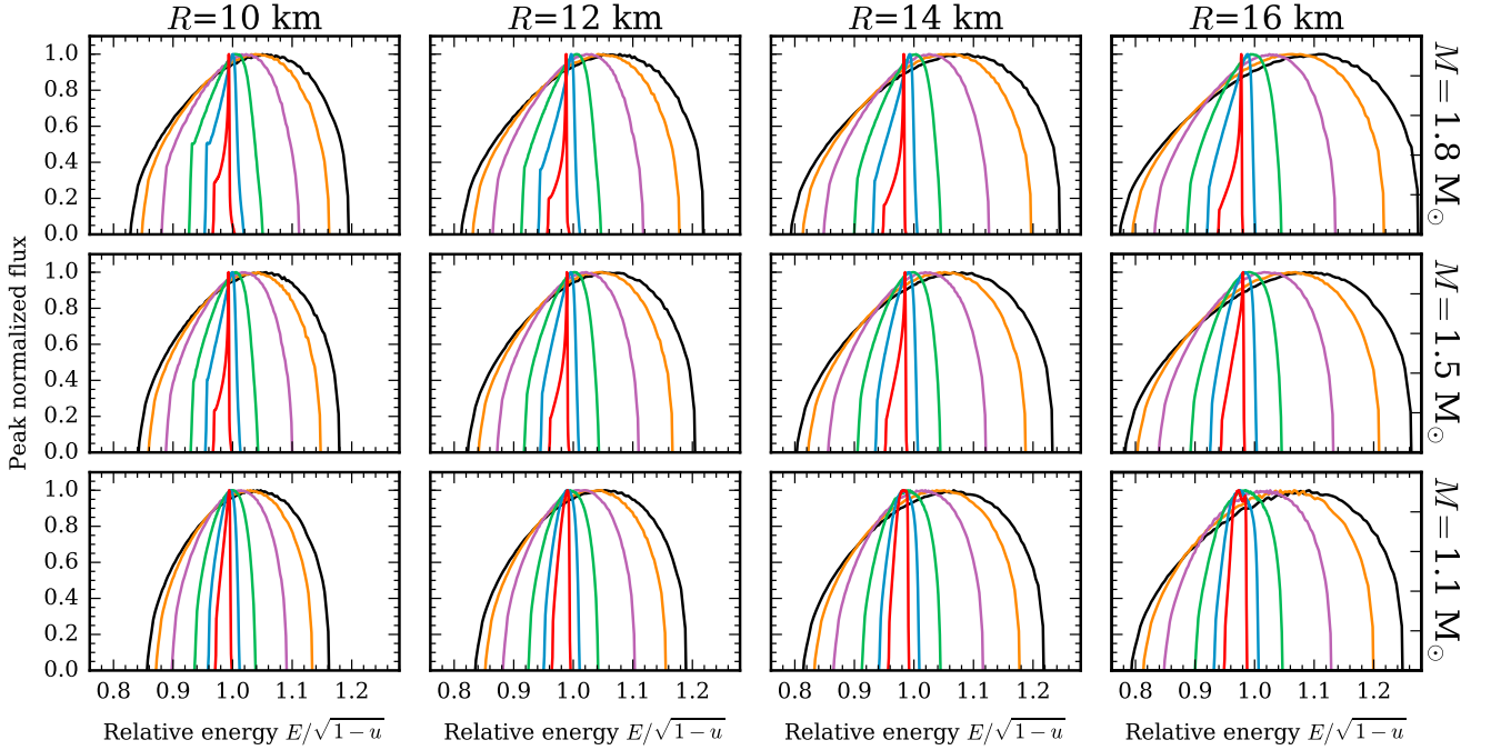
Fig. 6. Exact shapes of line profiles for different neutron stars spinning at 600Hz. Observer inclinations span a range from i = 5^\circ (red), 10^\circ (blue), 20^\circ (green), 40^\circ (purple), and 60^\circ (orange), to 90^\circ (black). The energy in the horizontal axis is scaled with the compactness \sqrt{1-u} = \sqrt{1-2GM/R_c} that would be expected from the gravitational redshift alone. Likewise, the flux in the vertical axis is always normalized with the peak flux to better show the evolution of the profile shape.
