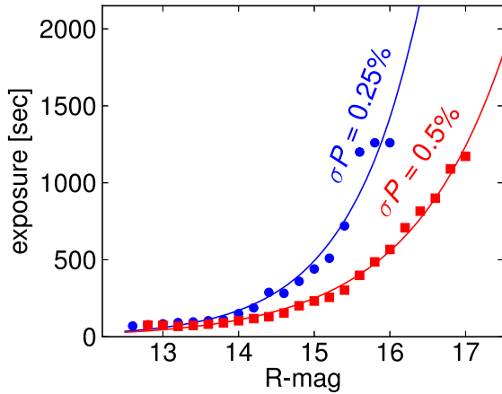
Figure 7. Required exposure time as a function of R -band magnitude in order to reach a \sigma_p of 0.25 per cent (blue) and 0.5 per cent (red). Squares and circles represent median values for multiple measurements obtained at different elevations, atmospheric conditions, and Moon phase. Curves show the exponential function fit to the data: a e^{bx} + c , with (a, b, c) = (3.2 \times 10^{-5}, 1.09, 39) and (0.0018, 0.79, -6) for a target \sigma_p of 0.25 per cent and 0.5 per cent, respectively.
