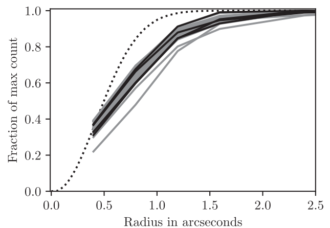
Figure 6. Fraction of total energy that is enclosed within an aperture of given radius (growth curve). The dotted line is the predicted curve from the Zemax software for a source at the center of the field (there is no significant difference between predictions for different spots of the same source). Solid grey lines show the observed growth curves for six sources located throughout the FOV (a separate curve is shown for each of the four spots), while the solid black lines are for a source in the centre of the field (within the mask).
