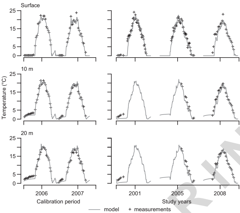
Fig. 1. Measured (crosses) and MyLake-simulated (line) temperatures at different water depths for Pyhäjärvi. Years 2006 and 2007 were used for calibration of the model.
