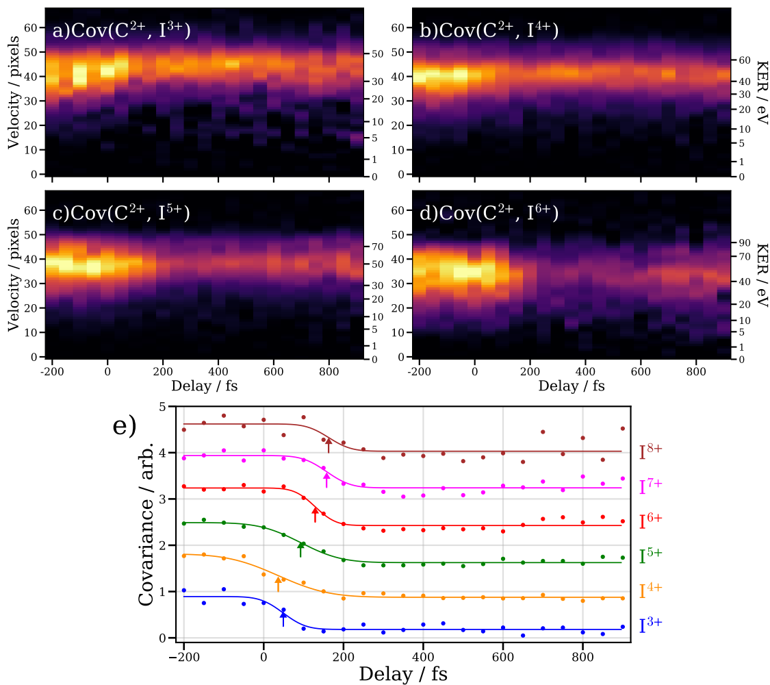
Fig. 12 Delay-dependent velocity distributions extracted from recoil-frame covariance maps between the C 2+ ions and a) I 3+ , b) I 4+ , c) I 5+ and d) I 6+ . Panel e) displays the integrated covariance as a function of pump-probe delay for the C 2+ , I n+ ( n=3-8 ) ion pairs. These have been fit to a Gaussian CDF as described in the text, with the centres of the CDF fits marked by coloured arrows
