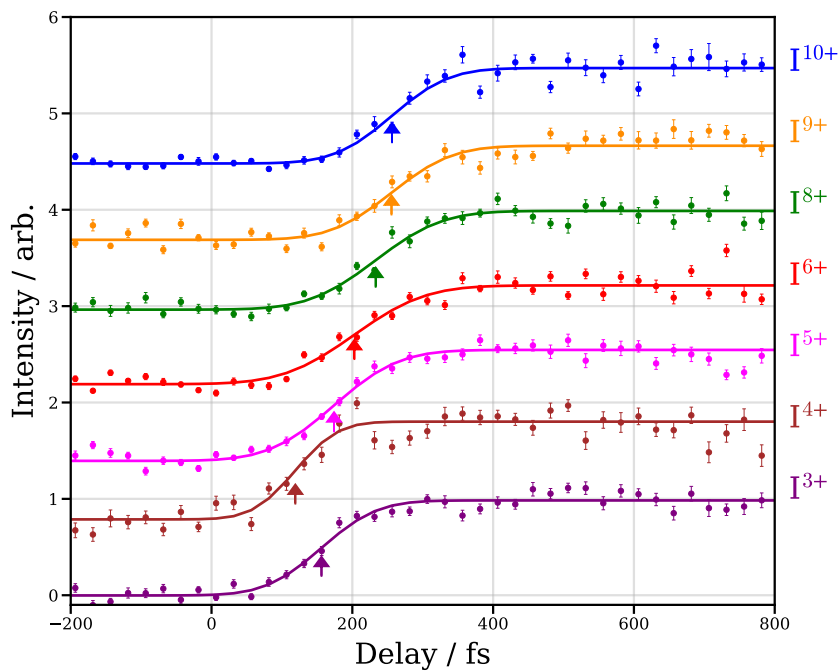
Fig. 5 Integrated ion yields as a function of pump-probe delay for Channel III for different iodine charge states, obtained by integrating the corresponding KER spectra below \sim 3.5\text{eV} . The data are quoted with standard errors determined from a bootstrapping analysis of the dataset. The data have been fit to a Gaussian cumulative distribution function, as described in the text. The centres of the CDF fits are marked with coloured arrows.
