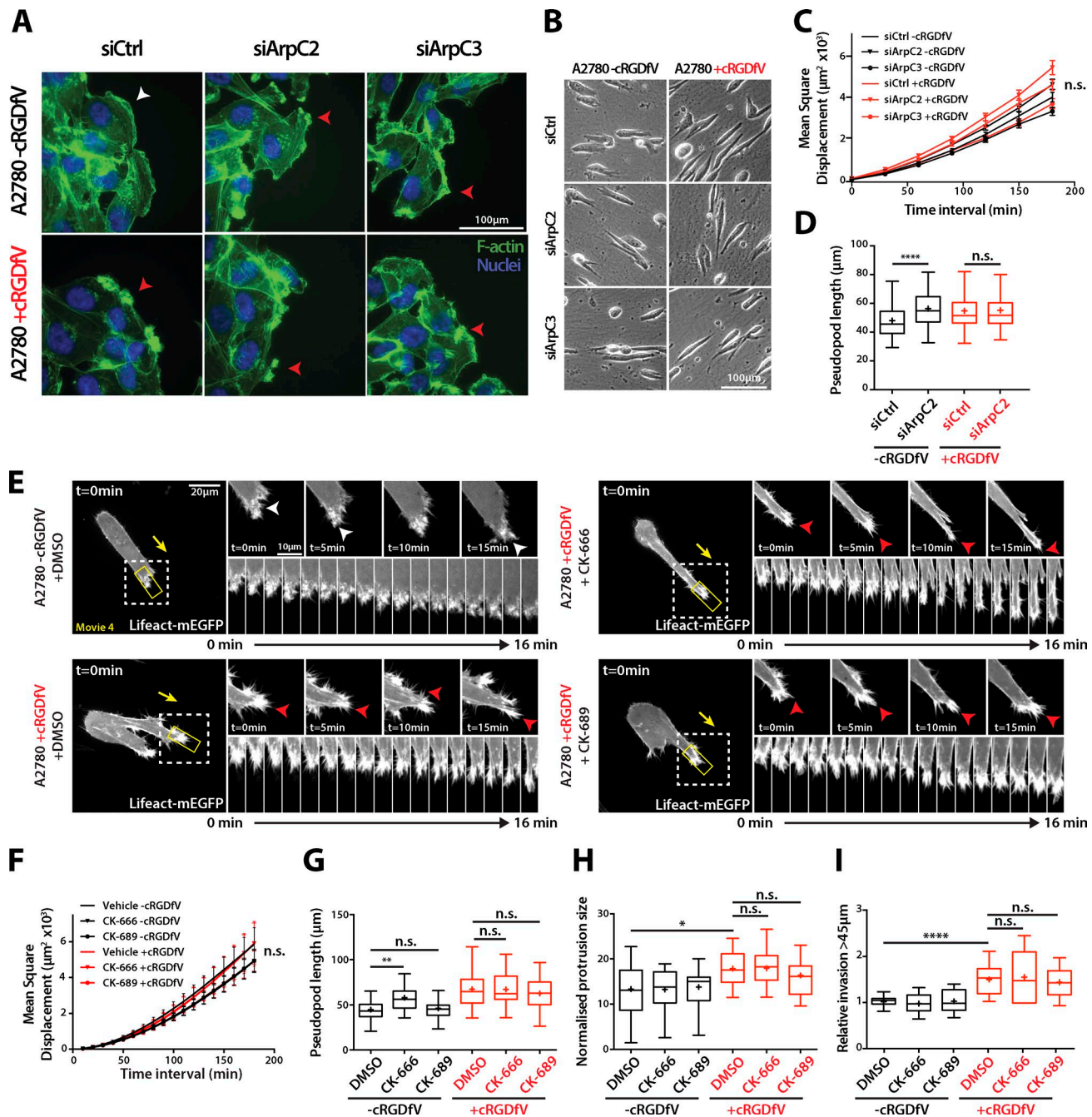
Figure 3. RCP- \alpha 5\beta 1 -driven migration and invasion is Arp2/3-independent. (A) siControl, ArpC2 knockdown, or ArpC3 knockdown A2780 cells were seeded onto glass coverslips, wounded after 24 h, and treated with cRGDFV (2.5 \mu\text{M} ) as indicated before fixation. F-actin was stained with FITC-phalloidin and nuclei with DAPI. The white arrowhead indicates lamellipodia; red arrowheads indicate nonlamellipodial ruffling protrusions. (B) siControl, ArpC2 knockdown, or ArpC3 knockdown A2780 cells were seeded onto 3D CDM for 4 h and treated with cRGDFV (2.5 \mu\text{M} ) where indicated before time-lapse imaging. (C) MSD measurement of siCtrl, siArpC2, and siArpC3 A2780 cells migrating in CDM. n \geq 99 cells per condition. (D) Pseudopod length of siCtrl and siArpC2 A2780 cells migrating in CDM. n = 100 cells per condition. (E) A2780 cells transiently transfected with Lifeact-mEGFP were seeded onto 3D CDM for 4 h, and treated with cRGDFV (2.5 \mu\text{M} , >2 h) and the indicated inhibitors (50 \mu\text{M} ) or vehicle control immediately before imaging. Maximum z projections are shown. White arrowheads indicate lamellipodia; red arrowheads indicate ruffling actin spikes. The white boxed regions are enlarged on the right, and the kymograph images are taken from the yellow boxed regions. Yellow arrows indicate the direction of migration. (F and G) MSD (F; n = 20 ) and pseudopod length (G; n = 50 ) of DMSO, CK-666, and CK-689-treated A2780 cells migrating in CDM. (H) Normalized protrusion size of A2780 cells expressing Lifeact-mEGFP treated with the indicated inhibitor (50 \mu\text{M} ) as in E. n = 13 –21 cells per condition with n \geq 25 frames quantified per cell. (I) A2780 cells were seeded into an inverted invasion assay in the presence of cRGDFV (2.5 \mu\text{M} ) where indicated for 72 h. DMSO, CK-666 (50 \mu\text{M} ), and CK-689 (50 \mu\text{M} ) were added 24 h after seeding and imaged 48 h later to quantify invasion. All data represent at least three independent experiments. Statistical significance was evaluated using ANOVA/Tukey's multiple comparison test. +, mean; n.s., not significant; *, P < 0.05 ; **, P < 0.01 ; ****, P < 0.0001 . Error bars represent the SEM.
