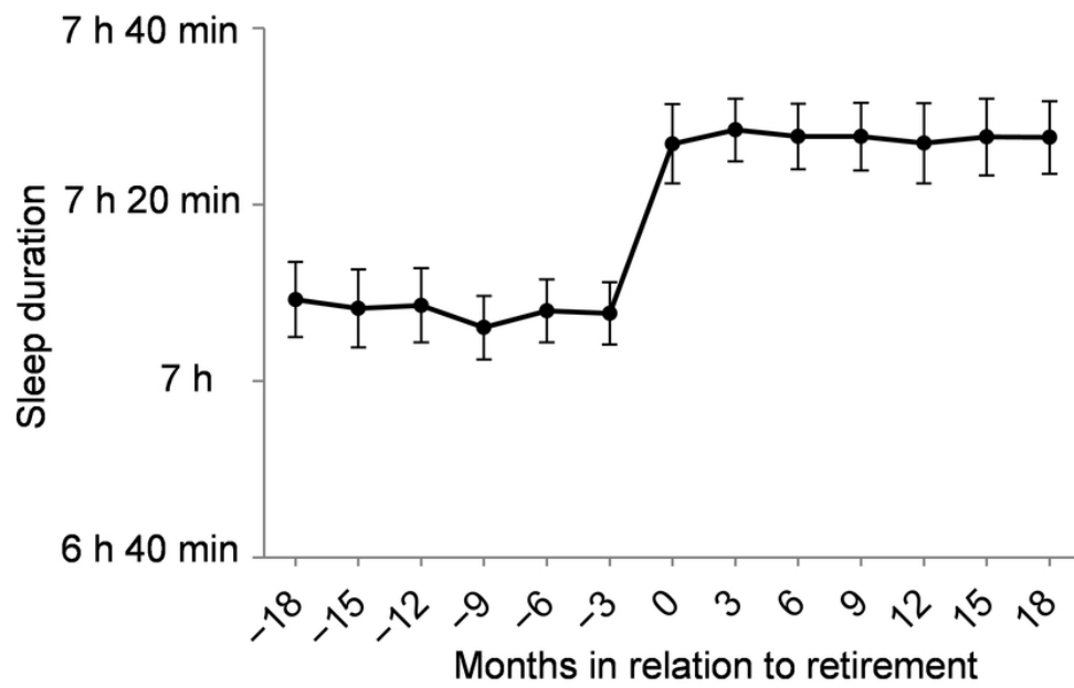
Figure 1 – Observed average sleep duration and its 95% confidence intervals per 24 hours in relation to retirement. The curve has been smoothed using moving averages.
