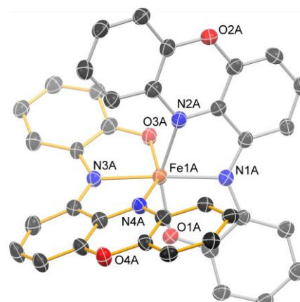
Figure 3. The molecular structure of 2 determined by single crystal X-ray at 120 K. Only one of the two discrete molecules in the asymmetric unit is drawn. Displacement ellipsoids are presented at 50% probability level. tert -Butyl groups and C–H atoms are omitted for clarity. Fe1A–O1A = 1.998(3), Fe1A–O3A = 2.013(3), Fe1A–N1A = 2.079(4), Fe1A–N2A = 2.133(4), Fe1A–N3A = 2.075(4), Fe1A–N4A = 2.145(4).
