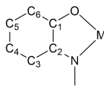
Figure 2. Comparison of o -amidophenoxide bonding parameters between 1 (Fe) and Ni(HL) 2 (from ref. 42). Bond lengths are reported in Å for both discrete o -amidophenoxide moieties of each complex.
