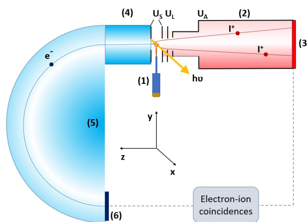
Fig. 1 Schematics of the electron-ion coincidence experiment at the Gas-phase Endstation. The labeled main components: (1) sample crucible and inlet, (2) ion TOF spectrometer, (3) ion detector, (4) electron lens, (5) electron analyzer and (6) electron detector. The components and voltages U_S , U_L and U_A are described in more detail in section 2.
