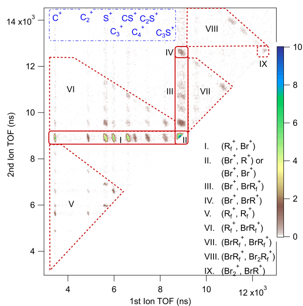
Fig. 3 Br 3d photoelectron PIPICO map with false coincidence background removed. Areas with notable patterns are highlighted in red. Areas with solid highlight (I-IV) contain the strongest patterns based on ion pair analysis while dashed areas (V-IX) belong to less important branches of the main dissociation tree. The blue labels mark vertical regions corresponding to the named ring fragment R_f^+ .
