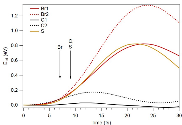
Fig. 12 Dicationic ground state energy after molecular dynamics in a core-hole state and Auger decay, with zero corresponding to the energy in the initial neutral ground state geometry. The arrows mark the core-hole lifetimes.
