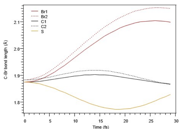
Fig. 11 Changes in the C-Br bond length during the molecular dynamics of the core-hole state. Legend indicates the atom with the core hole (the numbered atomic sites are presented in Fig. 2) and in each case, the length of the C-Br bond closest to the core hole is shown.
