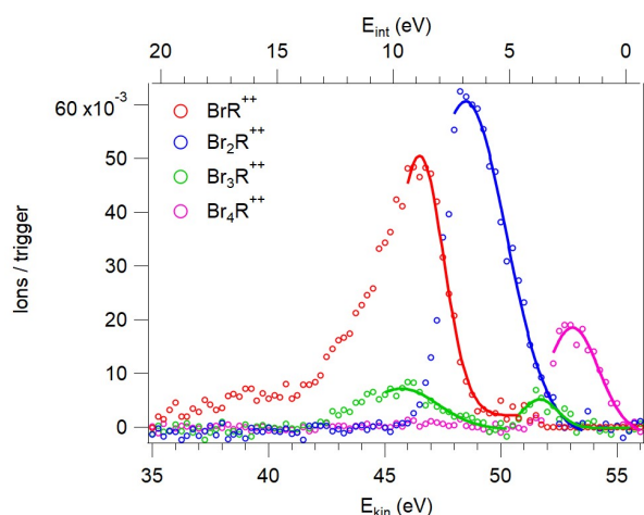
Fig. 5 CIYs of doubly charged ions as a function of the kinetic energy of the Br M_{4,5}V^{-2} Auger electron. False coincidence background has been subtracted using random-triggered events. The fitted Gaussians (solid lines) are used to determine appearance energies of each dication and the appearance of doubly charged parent marks the zero of internal energy (top axis) as stated in eqn (3). Br_3R^{++} apparently forms two distinct peaks but the left peak is most likely due to imperfect filtering as explained in the text.
