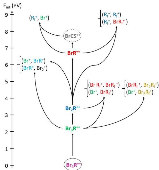
Fig. 8 Proposed general main dissociation tree for the doubly charged parent molecule. All neutral fragments are omitted, and the colors refer to Fig. 5 and 6. Dications and cation pairs are placed at their appearance energies (determined from Fig. 5 and 6) and the arrows indicate the main dissociation pathways. Several minor dissociation pathways are not shown. The existence of the intermediary product BrCS^{++} was deduced from the slope analysis of the PIPICO data.
