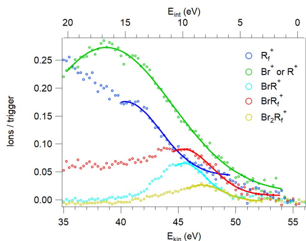
Fig. 6 CIYs of cation groups as a function of the kinetic energy of Br M_{4,5}NN Auger electron after subtraction of the false coincidence background and the ion yield from processes other than the Br M_{4,5}V^{-2} Auger decay. The fitted Gaussians (solid lines) are used to determine appearance energies of each group. Due to presence of unwanted background, only the steeply rising part of R_f^+ CIY is fitted, which leads to high base level for the Gaussian.
