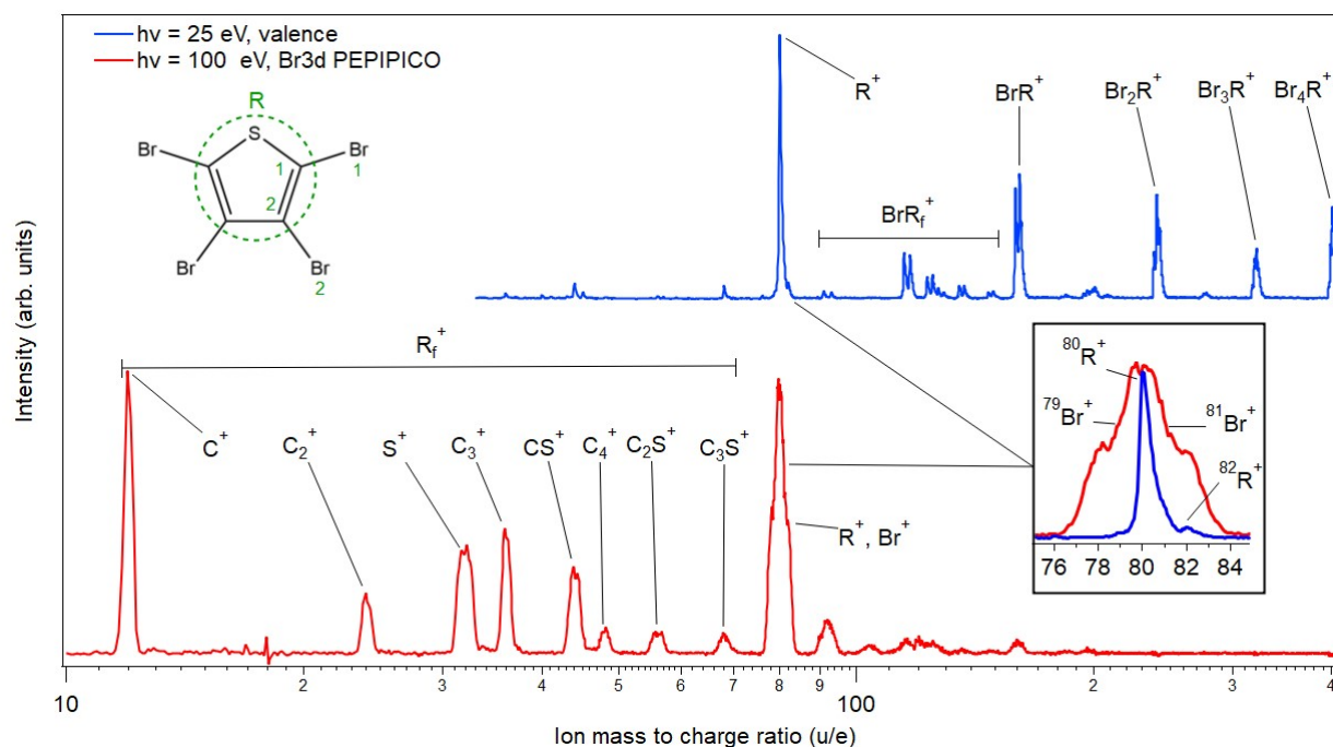
Fig. 2 Ion mass spectra with valence ionization (blue) and from Br 3d PEPICO measurement (red) on logarithmic scale. The contribution of false coincidences has been removed. The left side of the valence TOF is cropped out due to contribution of the rest gas and lack of peaks from the sample. The feature at m/z \approx 80 u/e is much broader in the Br 3d ionization than in the valence ionization due to presence of \text{Br}^+ ions (inset). Symmetrically unique Br and C atoms have been numbered for later use.
