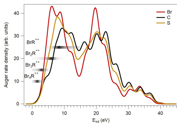
Fig. 10 Simulated population curves of the dicationic states for different core-hole sites of \text{Br}_4\text{R} as a function of internal energy of the Auger final state relative to V_{DIP} . The graphs are normalized to the same area. The final-state energy ranges producing \text{Br}_x\text{R}^{++} dicationic species are indicated by gray shading.
