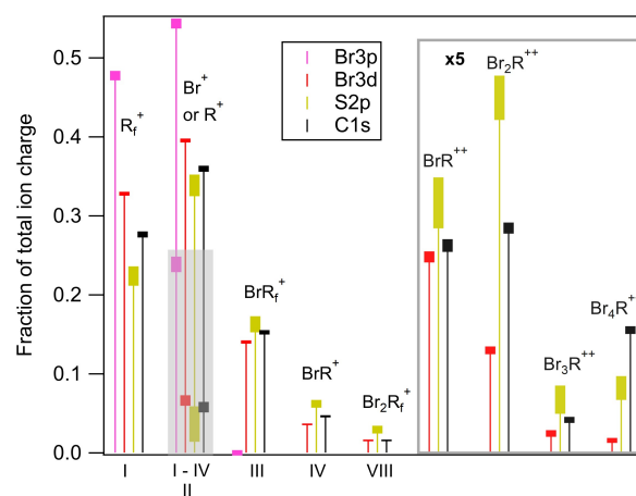
Fig. 9 Fractions of total released charge carried by various singly and doubly ( \times 5 ) charged ions, measured in coincidence with inner-shell photoelectrons from Br, S and C atoms. The lower markers on the ( \text{Br}^+ or \text{R}^+ ) ion bar within the gray area denote the estimated fraction of the ions that come from the ( \text{Br}^+ , \text{R}^+ ) and ( \text{Br}^+ , \text{Br}^+ ) dissociation channels (see text for details). Error limits are marked by the thick regions of the bars. Roman numerals under the ion fractions refer to the regions in the PIPICO map (Fig. 3) from which the major contribution of the ions comes from.
