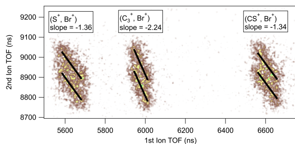
Fig. 4 The region of the PEPICO map with the strongest ( R_f^+ , Br^+ ) patterns in area I of Fig. 3 excluding ( C^+ , Br^+ ). The patterns for ( S^+ , Br^+ ), ( C_3^+ , Br^+ ) and ( CS^+ , Br^+ ) are marked with two black lines due to two bromine isotopes. The slopes of the lines are marked above. A smaller 2D bin size was used than in Fig. 3.
