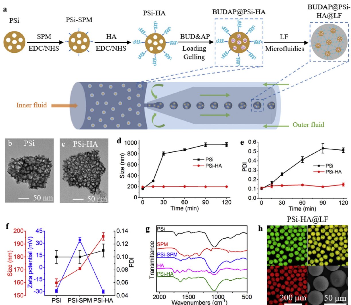
Fig. 2. a) Fabrication process of hierarchical structured and programmable responsive vehicles (BUDAP@PSi-HA@LF). b–c) Transmission electron microscopy (TEM) image of b) PSi and c) PSi-HA. d) Size and e) polydispersity index (PDI) of PSi and PSi-HA dispersing in Milli-Q water during 2 h, demonstrating the high colloidal stability of PSi-HA over time. Data represent mean \pm SD. ( n = 3 ). f) Size, PDI, and surface zeta potential of PSi, PSi-SPM and PSi-HA. g) FTIR of PSi, SPM, PSi-SPM, HA and PSi-HA. h) The monodispersity of the fabricated BUDAP@PSi-HA@LF was studied by confocal microscopy and SEM. PSi-HA was conjugated with FITC and LF layer was labelled with TRITC. The confocal images showed the FITC (green), TRITC (red) and the overlay (yellow) channels. The surface of the particles was observed by SEM. (For interpretation of the references to color in this figure legend, the reader is referred to the Web version of this article.)
