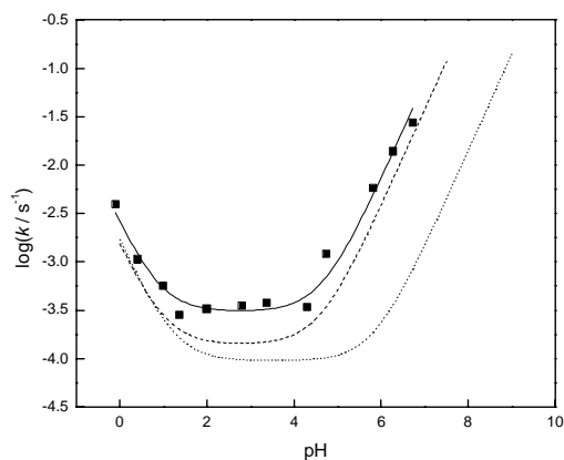
Fig. 1 pH-rate profile for the cleavage of 1a and 1b (■), 2 (dashed line) and 3 (dotted line) at 25.0 °C, I(\text{NaNO}_3) = 1.0 \text{ mol L}^{-1} .
