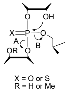
Scheme 1 Cleavage of a trinucleoside monophosphate or phosphorothioate via P-O5' (Route A) or P-O3' (Route B) fission.
