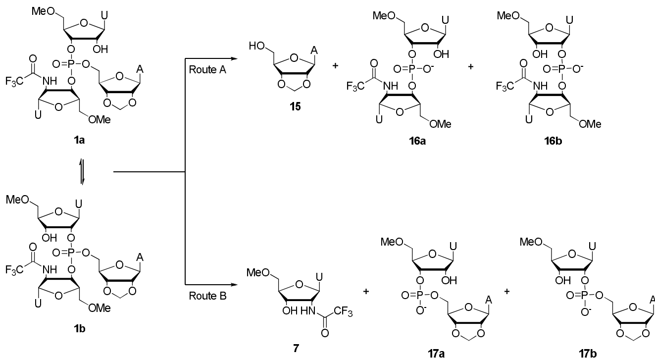
Scheme 3 Hydrolytic reaction pathways of 1a and 1b .
