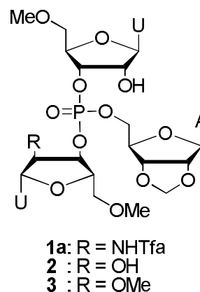
Scheme 1 Cleavage of a trinucleoside monophosphate or phosphorothioate via P-O5' (Route A) or P-O3' (Route B) fission.
