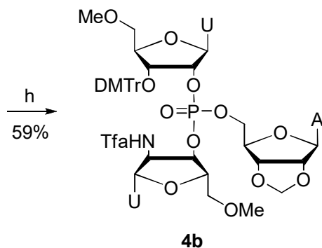
Scheme 2 Preparation of the trinucleoside 2',3',5'-monophosphate 4b . Reagents and conditions: (a) \text{NaN}_3 , DMF, (b) (1) \text{Ph}_3\text{P} , pyridine, (2) aq. \text{NH}_3 , pyridine, (c) S -ethyltrifluoroacetate, MeOH, (d) (\text{Me}_2\text{N})_3\text{P} , 1 H -tetrazole, MeCN, (e) 7 , 1 H -tetrazole, MeCN, (f) 5'- O -methyl-3'- O -(4,4'-dimethoxytrityl)uridine, 1 H -tetrazole, MeCN, (g) \text{I}_2 , THF, \text{H}_2\text{O} , 2,6-lutidine, (h) \text{NH}_3 , MeOH.
