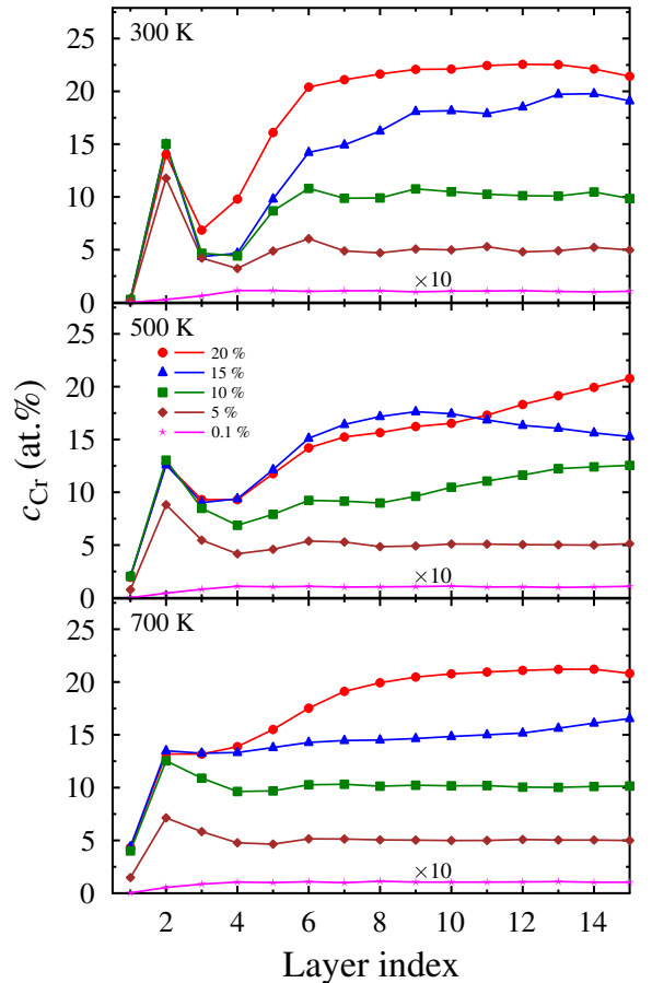
FIG. 7. (Color online) Chromium concentration depth profiles for different average chromium concentrations and simulation temperatures. Curves for 0.1 % are multiplied by 10 for better visibility.
