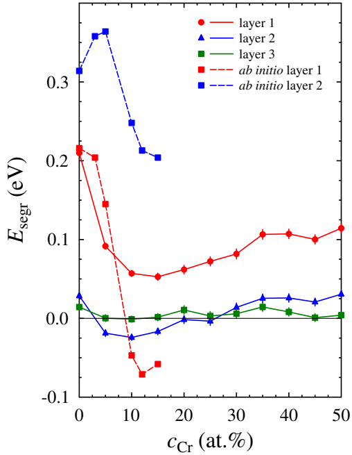
FIG. 4. (Color online) Segregation energy of the three near surface atomic layers as a function of bulk Cr concentration as predicted by the 2BEAM model. The ab initio data is the one presented in Table I.
