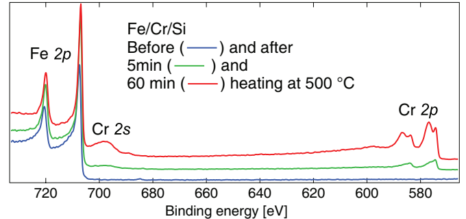
FIG. 12. (Color online) Overview HAXPES spectra of the Fe/Cr bilayer sample measured with 2300 eV photon energy before and after two heating treatments. In addition to the Cr 2s and Cr 2p spectra appearing after annealing, the increased intensity of Cr 2p as a comparison to Fe 2p after different annealing times demonstrates the Cr diffusion towards the surface. The intensity of Fe 2p 3/2 of the presented spectra is normalized to one after setting background to zero.
