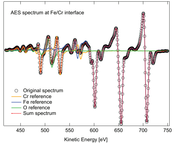
FIG. 10. (Color online) Example of an AES spectrum of Fe/Cr interface (o curve) of Fe/Cr/Si sample. The sum spectrum (dashed curve) was obtained by Principal Component Analysis (PCA) of Casa XPS 2.13.16. 63
