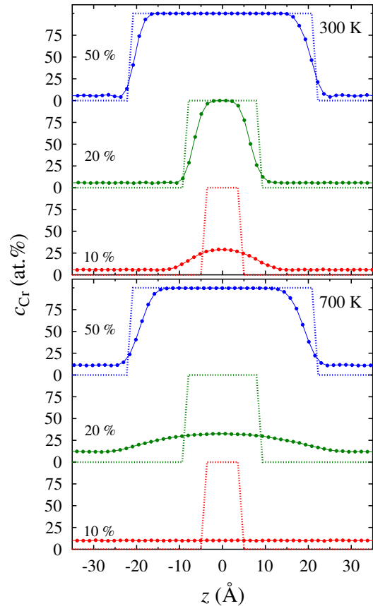
FIG. 9. (Color online) Cr concentration profiles for the layer widths corresponding different total Cr concentrations simulated in different temperatures. Thin dashed lines show the initial Cr profile.
