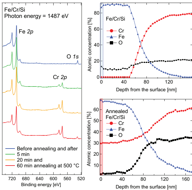
FIG. 11. (Color online) Left hand side presents the Fe 2p, Cr 2p and O 1s XPS spectra of a Fe/Cr bilayer sample before (topmost spectrum) and after annealing. These spectra were measured using Al K\alpha twin anode. Photoemission spectra clearly demonstrate the increase of Cr 2p intensity as a function of annealing time confirming the Cr diffusion into the Fe layer. The upper AES profile on the right is taken over the Fe/Cr interface before any heating was carried out starting sputtering from the surface represented by upper most XPS spectrum (blue) on the left. The lower AES depth profile on the right was taken after all the heating treatments starting from the surface concentration presented in the lowest (red) XPS spectrum on the left.
