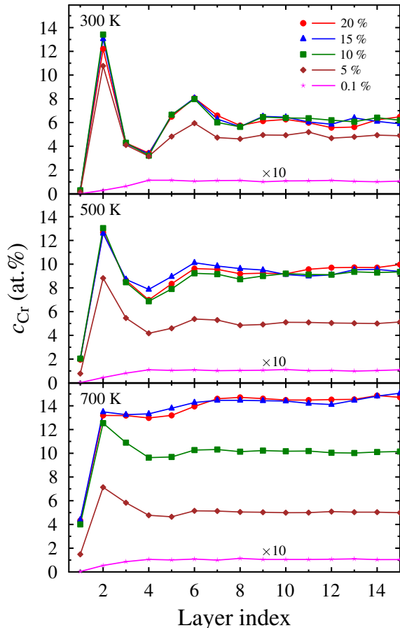
FIG. 8. (Color online) As in Fig. 7 but with chromium precipitates removed. Removing was done by only taking into account atoms whose average type during the last 60000 simulation steps was smaller than 1.5 where value 1.0 corresponds to pure Fe and 2.0 to pure Cr.
