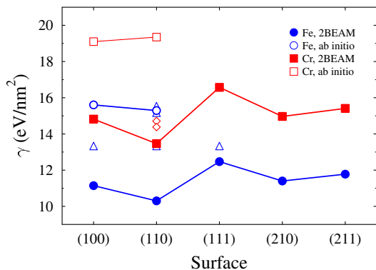
FIG. 2. (Color online) Surface energies of low index surfaces of bcc iron and chromium as predicted by the 2BEAM model. Results of ab initio calculations (open circles for Fe and open squares for Cr) are from Ref. 58. Experimental values (open triangles for Fe and open diamonds for Cr) are from Ref. 60.
