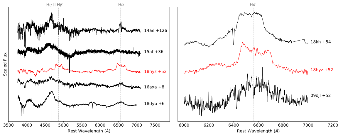
Figure 12. TDE candidates with similar spectral features to AT2018hzy. Left: TDEs with flat Balmer decrements. Also note the late appearing He II in 14ae. Right: TDEs which may show disc-like profiles. 18hzy has the most obvious double peak.
