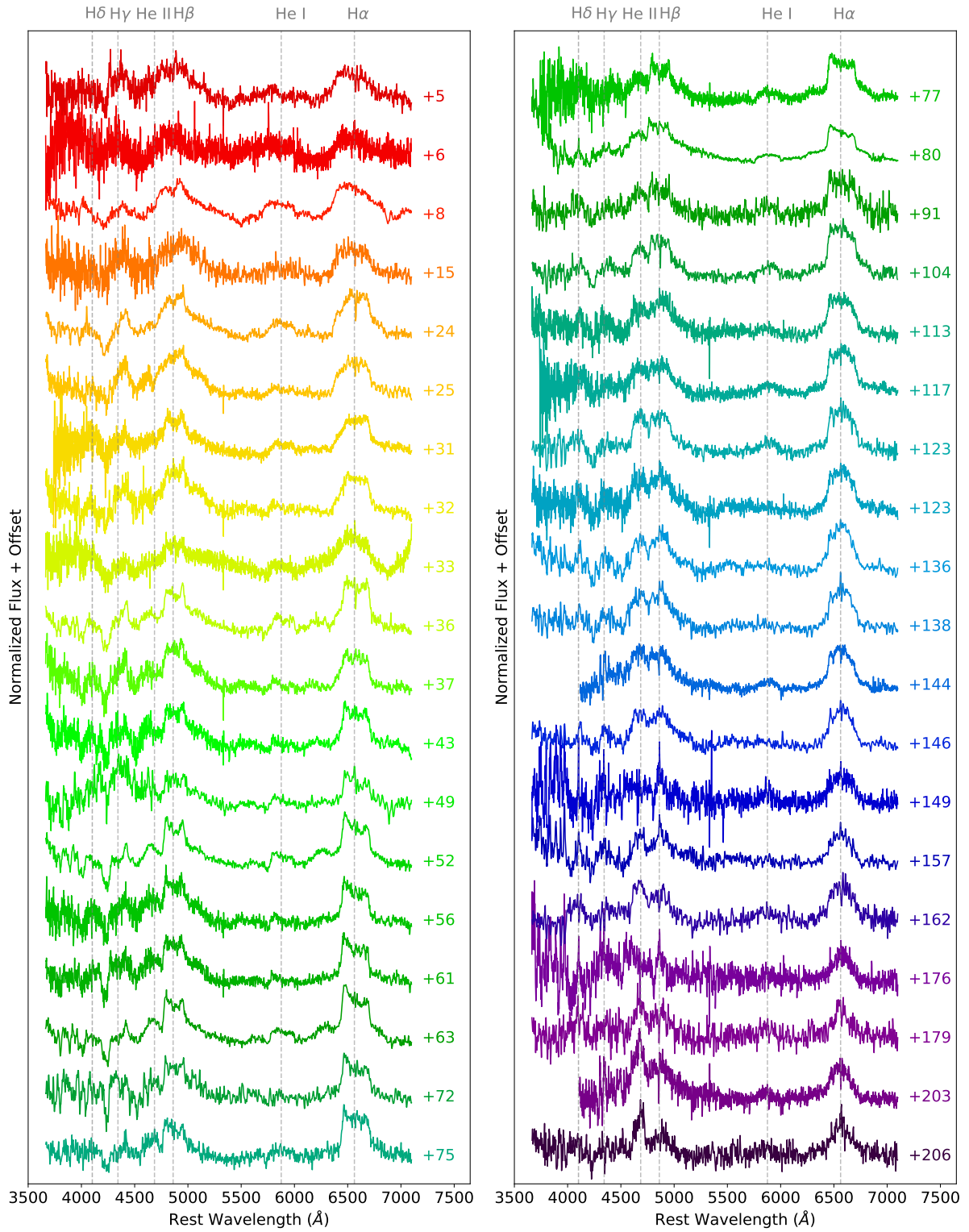
Figure 4. All host and continuum subtracted spectra. The days after peak in the TDE rest frame are marked on the right.
