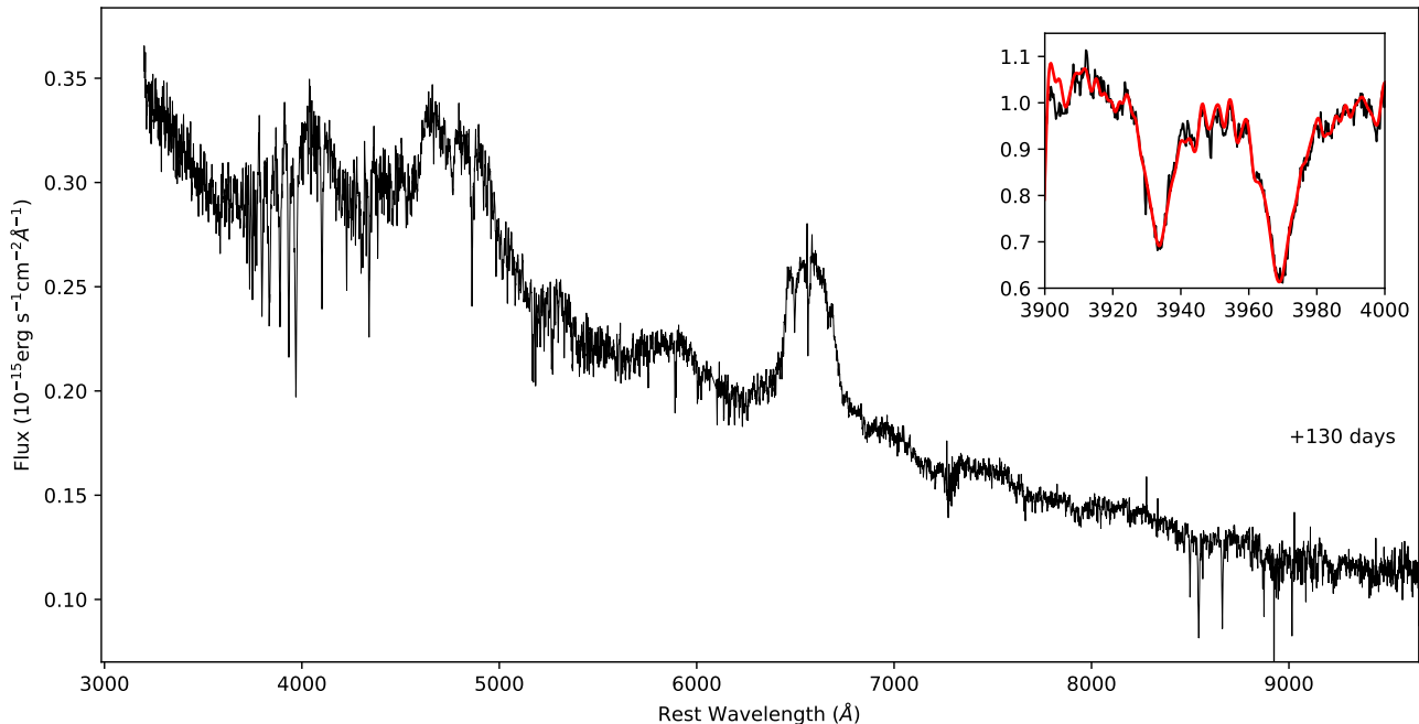
Figure 3. The X-Shooter spectrum of AT 2018hyz. Inset: The normalised X-Shooter spectrum (black) zoomed in on Calcium H and K absorption lines. The best fitting model is overlaid in red.
