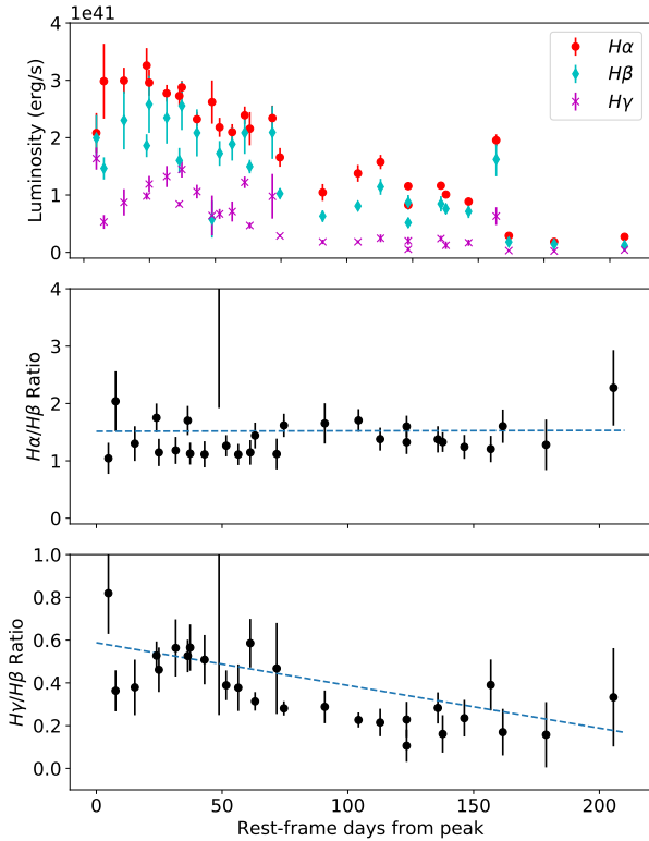
Figure 6. The H\alpha , H\beta and H\gamma luminosities fade with time (top), H\alpha/H\beta stays roughly constant (middle), while H\gamma/H\beta appears to decline. The dashed lines shows the line of best fit. The error bars are underestimated as they do not include systematics.
