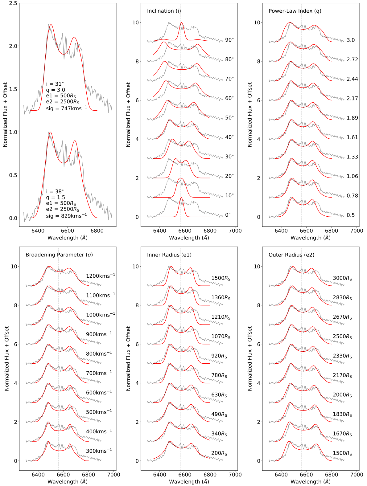
Figure 10. The top left panel shows examples of best fitting models to our spectrum. The remaining panels explore parameter space of the circular disc model. In each of these plots only one parameter is varied, while the others are fixed at i = 38^\circ , q = 1.5 , \sigma = 500\text{ km s}^{-1} , e_1 = 500R_S and e_2 = 2500R_S .
