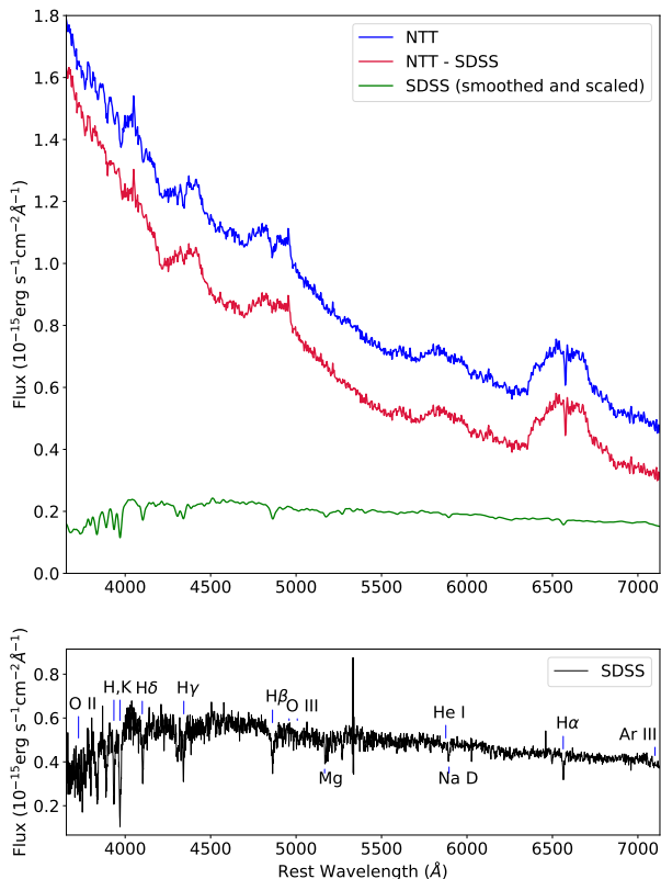
Figure 1. Lower: The original SDSS spectrum. Upper: (green) the SDSS spectrum degraded to match the resolution and scaled to the slit width of the NTT spectra, (blue) an NTT spectrum from 02/12/2018 and (red) the same NTT spectrum minus the degraded and scaled SDSS spectrum.
