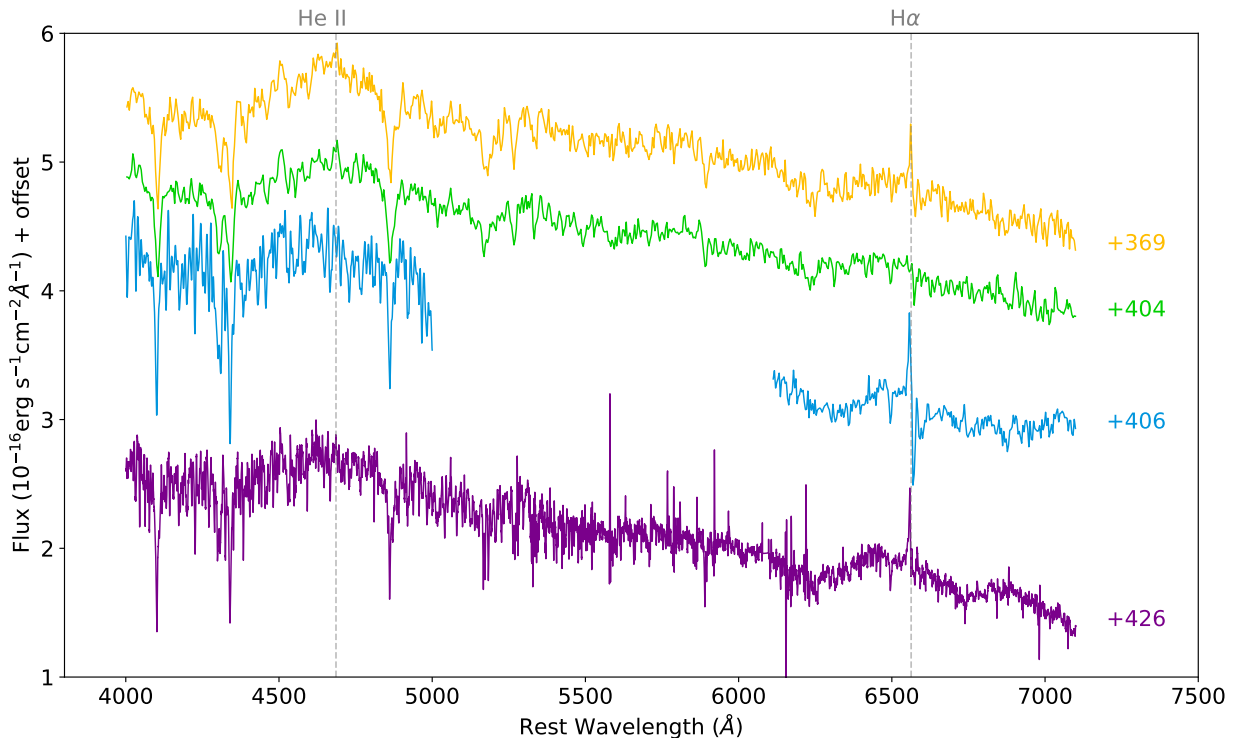
Figure 8. Late-time spectra taken once AT 2018hyz was no longer obscured by the Sun. The first two are from the NTT, the third from the WHT and the most recent is from X-Shooter. The host has not been subtracted from these spectra. A narrow H\alpha line has appeared and He II is just visible in the earliest of these spectra
