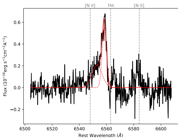
Figure 9. A two Gaussian component fit to the narrow H\alpha line in the X-Shooter spectrum taken +426 days from peak. The line appears blueshifted, with the narrow component centered on 6558 Å. The broad component might be [N II] \lambda 6548, with the corresponding [N II] \lambda 6584 to the right.
