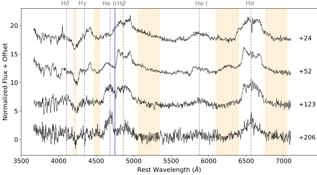
Figure 5. Continuum subtracted spectra from different epochs with emission lines labelled. The time after peak (in rest-frame days) when each spectrum was taken is marked on the right. The regions used in local continuum subtractions are highlighted in orange. After continuum subtraction the area between these regions was integrated to find the line flux, with the exception of H\beta , where the lower limit is the solid blue line to avoid He II.
