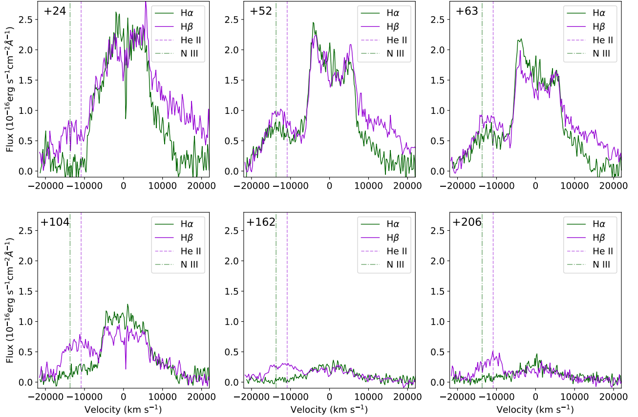
Figure 7. Velocity profiles of H\alpha and H\beta from six epochs (marked in the top left in rest-frame days from peak). At +52 days, the blue bump in H\alpha is at a similar velocity to what we had assumed to be He II, possibly suggesting a blue-shifted outflow ( \sim 12000 \text{ km s}^{-1} ). At +162 days a second peak appears on He II that matches the position of the N III line produced by Bowen fluorescence.
