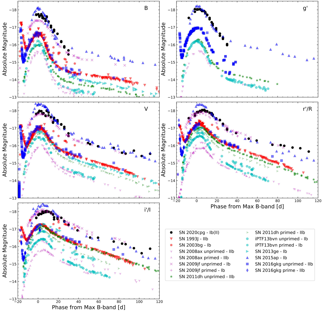
Figure 6. Comparison of the absolute magnitude light curves of several SNe Ib and Iib with SN 2020cpg. All photometry is relative to B_{\max} light which was either taken from the literature or by fitting a Gaussian to the B -band peak. The light curves have been corrected for time dilation as well as corrected for both Milky Way and host galaxy reddening when possible. Primed bands are SDSS photometry bands and unprimed are the Johnson-Cousins photometry bands. Error on absolute magnitudes not included.
