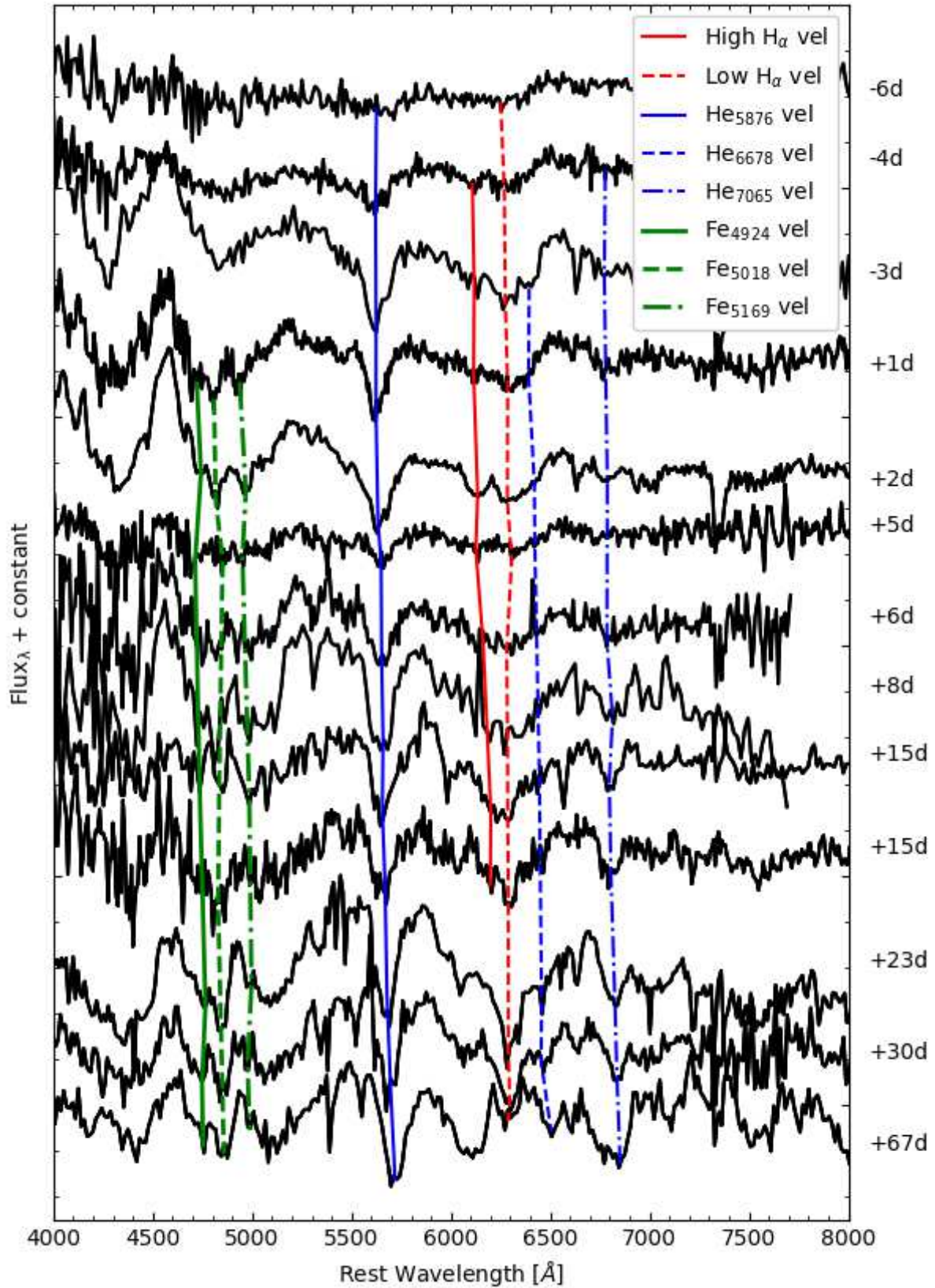
Figure 7. Evolution of SN 2020cpg spectra. The spectra have been plotted between 4000 – 8000 Å to highlight the regions where prominent H \alpha , He I and Fe II features are visible. The different elements are shown by the different lines, with H \alpha = red, He I = blue and Fe II = green, and different element lines given by different styles. Lines are only shown when line features are clearly visible within the spectra.
