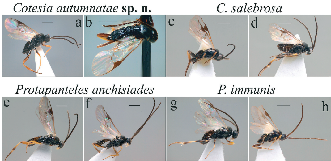
Fig. 7. Habitus of the four microgastrine species parasitizing Epirrita autumnata in Fennoscandia. In each pair, female (left) and male (right). Paratype for Cotesia autumnatae sp. n. Scales 1 mm.
