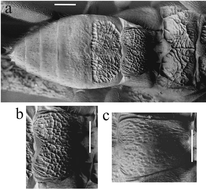
Fig. 3. – a. Propodeum and metasoma of Cotesia autumnatae sp. n., paratype female, dorsal. – b. Tergite 1 of C. autumnatae sp. n., paratype female, dorsal. – c. Tergite 1 of Cotesia jucunda , female, dorsal. Scales 0.2 mm.
