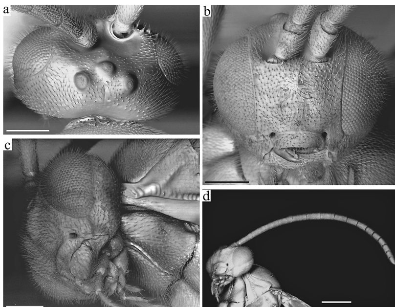
Fig. 2. Cotesia autumnatae sp. n., paratype female. – a. Head, dorsal. – b. Head, facial. – c. Head, antero-latero-ventral. – d. Antenna. Scales 0.2 mm, except 0.5 mm in d.
