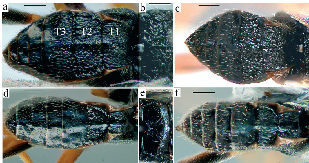
Fig. 8. – a. Metasoma of Cotesia salebrosa , with tergites 1–3 (T1–T3) indicated, female, dorsal. – b. Propodeum of C. salebrosa , female, dorsal. – c. Metasoma of C. autumnatae sp. n., paratype female, dorsal. – d. Metasoma of Protapanteles anchisiades , female, dorsal. – e. Propodeum of P. anchisiades , female, dorsal. – f. Metasoma of P. immunis , female, dorsal. Scales 0.2 mm.
