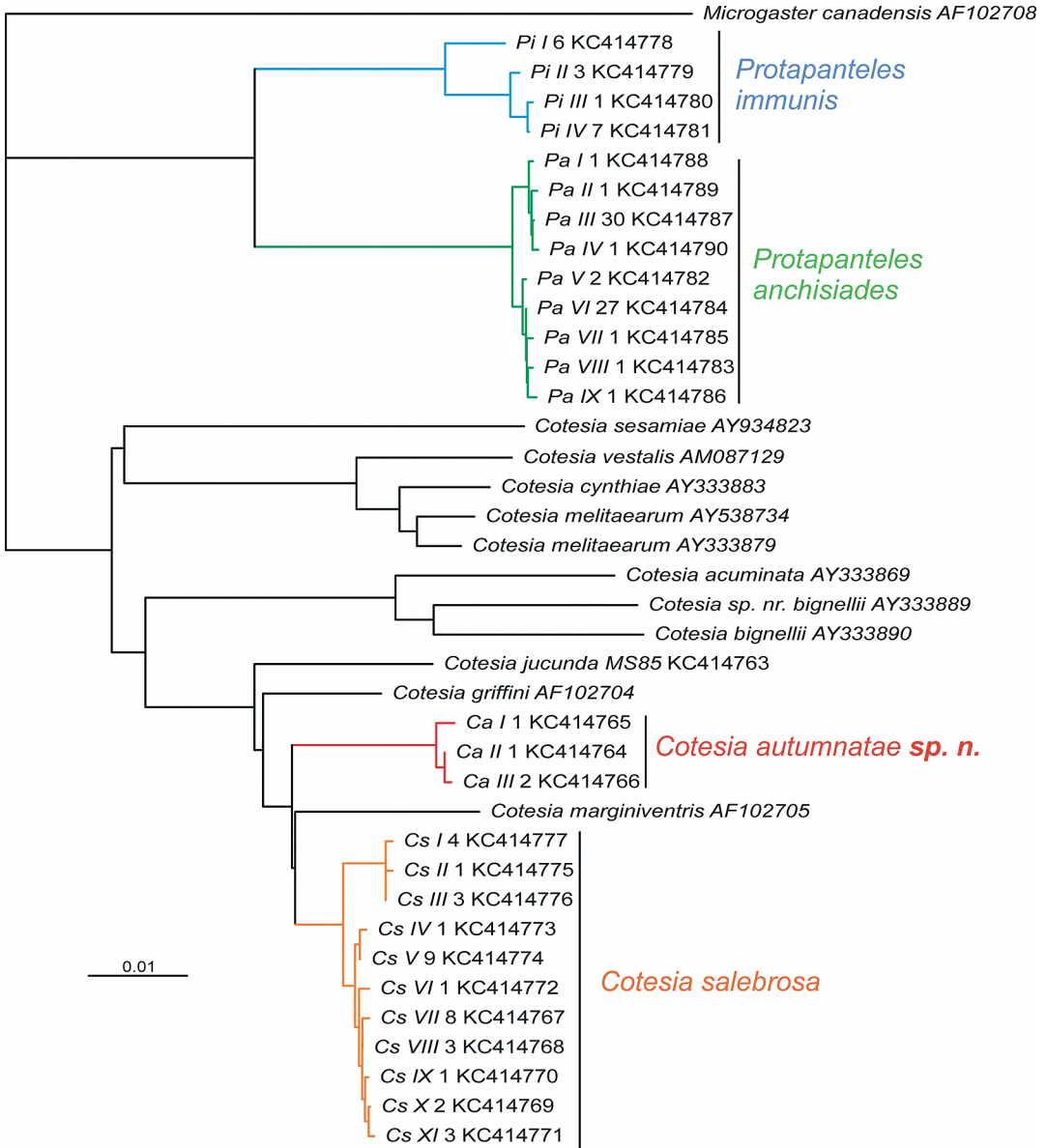
Fig. 1. The NJ dendrogram of COI haplotypes of four microgastrine species reared from larvae of the geometrid Epirrita autumnata in Fennoscandia. Cotesia jucunda , morphologically close to C. autumnatae sp. n., has also been included as well as other Cotesia spp. and, as an out-group, Microgaster canadensis . The GenBank accession number is given for each sequence used in the analysis. For each haplotype of the four species reared from E. autumnata , the number just before the GenBank accession number shows the number of specimens in that haplotype; information of all specimens are listed in Table 2. Scale gives percentage divergence based on Kimura 2-parameter model corrected genetic distances.
