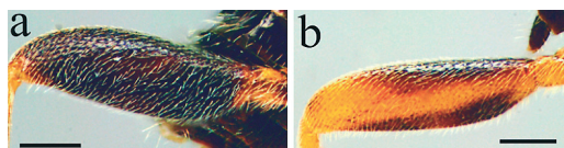
Fig. 9. – a. Hind femur of Cotesia salebrosa , female, lateral. – b. Hind femur of C. autumnatae sp. n., paratype female, lateral. Scales 0.2 mm.
