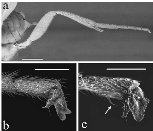
Fig. 5. – a. Hind leg of Cotesia autumnatae sp. n., paratype female, lateral. – b. Apical segment of front tarsus of C. autumnatae sp. n., paratype female, lateral. – c. Apical segment of front tarsus of C. jucunda , female, lateral. Scale 0.5 mm in a, 0.1 mm in b and c.
