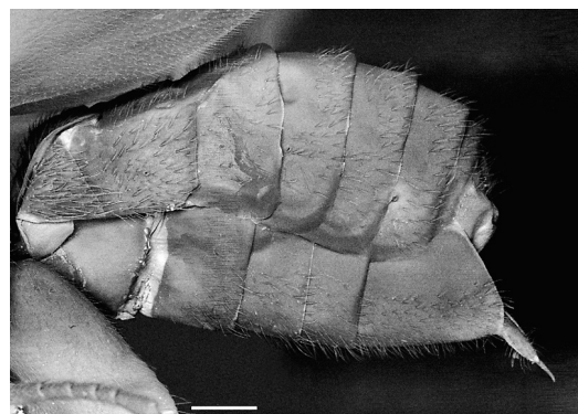
Fig. 6. Metasoma of Cotesia autumnatae sp. n., paratype female, lateral. Scale 0.2 mm.
