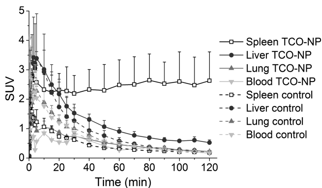
Figure 4. TACs for blood, spleen, liver, and lungs for animals injected with TCO-NPs (0.2 mg/animal) 15 min before injecting [ 18 F]1 ( n = 2). The control animals were injected only with [ 18 F]1 ( n = 2).
