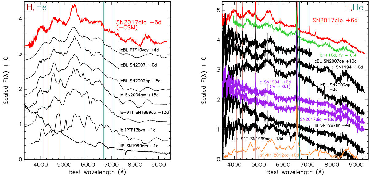
Figure 3. (Left) Comparison of the CSM interaction-subtracted spectrum of SN 2017dio (red) with spectra of other SNe (black; including SNID templates of Modjaz et al. 2014). (Right) Comparison of the +6 days spectrum of SN 2017dio (red) with those of other SNe combined with interaction spectrum (black; f_V = 0.3 ), a template SN Ic+CSM interaction spectrum from Leloudas et al. (2015, green), and SN 2012ca (orange). The spectrum of SN 1994I combined with interaction spectrum ( f_V = 0.1 ) is shown for comparison with SN 2017dio at +18 days. The comparison spectra are from WISerEP. In both panels, phases are days from maximum for spectra other than SN 2017dio.
