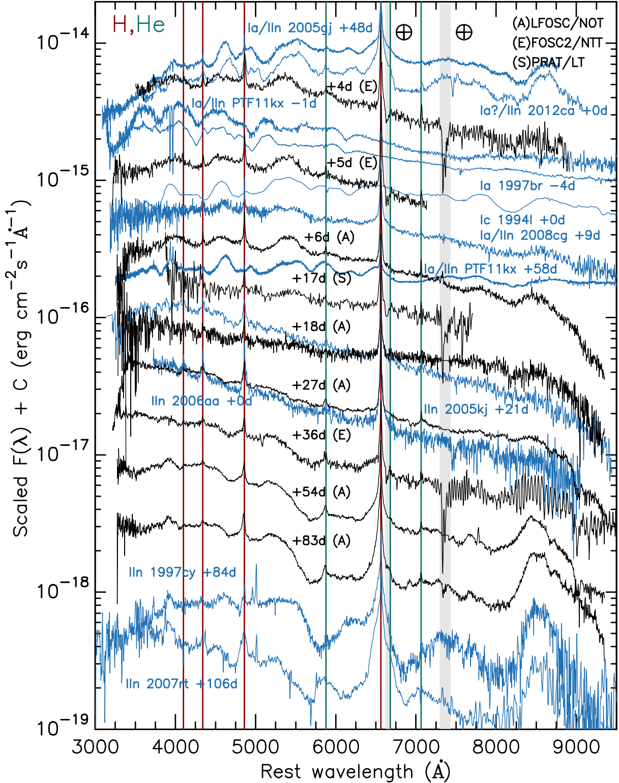
Figure 1. Spectral sequence of SN 2017dio. Comparison spectra of other SNe (obtained through WISeREP c , Yaron & Gal-Yam 2012) are plotted in blue. Phases for SN 2017dio are days after the discovery, while for other SNe phases are post maximum. The rest wavelengths of the H I lines are indicated with dark red and He I with dark green lines. Telluric absorption regions in SN 2017dio spectra are indicated with grey shade. SN 2017dio spectra will be made publicly available at WISeREP and the Open Supernova Catalog d (Guillochon et al. 2017).
