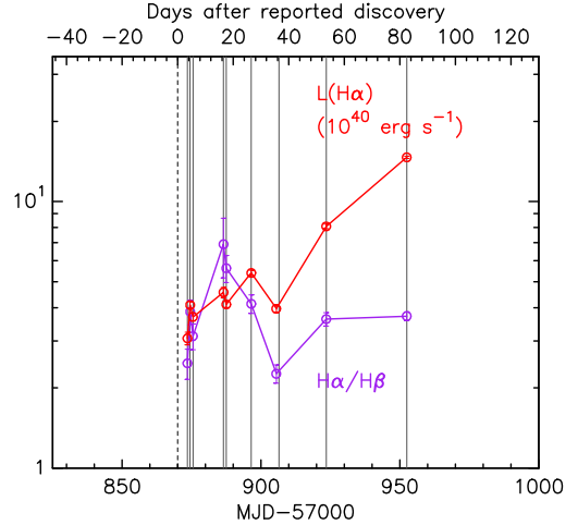
Figure 5. The evolution of the H\alpha/H\beta flux ratio (purple), and H\alpha line luminosity (red).
