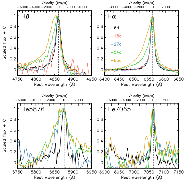
Figure 4. The observed line profile evolution for H\alpha , H\beta , He I \lambda 5876 , He I \lambda 7065 . Only data taken with the same instrument and setting (ALFOSC) are plotted, for clarity.
