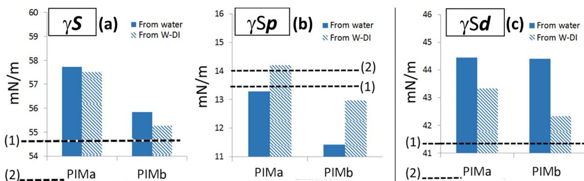
Figure 4. Wu's model estimations of (a) \gamma_S and its (b) polar component ( \gamma_{Sp} ) and (c) dispersive component ( \gamma_{Sd} ) of films made of PIMa and PIMb, processed from water (solid color bars) or W-DI (dash-patterned bars). Dashed horizontal lines indicate the SFE, SFE p , and SFE d values of the blank surfaces of (1) plasma glass and (2) glass-water.
