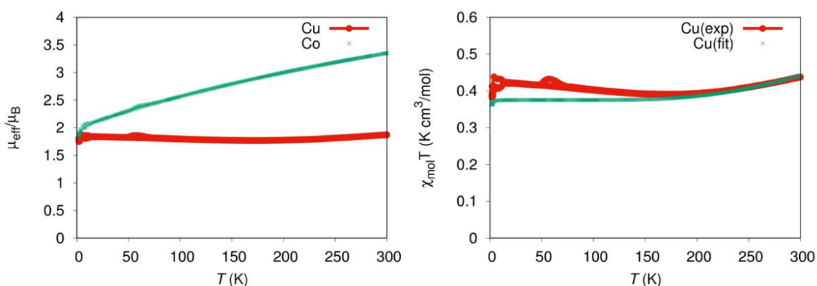
Figure 3 Left: The \mu_{\text{eff}} vs. T plots for [\text{CoL}^*_2] (upper line) and [\text{CuL}^*_2] (lower line). Right: The experimental (upper line) and fitted (lower line) \chi_{\text{mol}}T vs. T plot for [\text{CuL}^*_2] in cgs units. The bulges seen at ca. 60 K, are due to some air in the SQUID instrument. The discrepancy in \chi_{\text{mol}}T vs. T plot at lower temperatures is mostly due to the sample holder.
