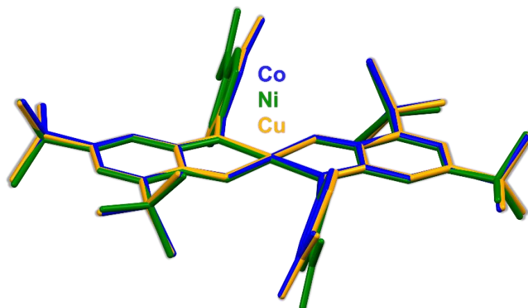
Figure 1 Comparison between the geometries of molecular units in crystal structures of [ML^*_2] [ M = Co (blue), Ni (green) and Cu (yellow)].
