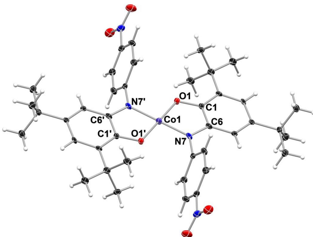
Figure 2 The complex unit in the crystal structure of [CoL^*_2] . Thermal ellipsoids are drawn at the 30% probability level.
