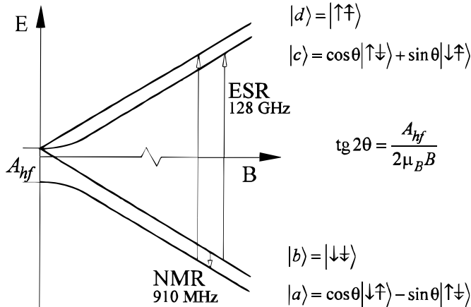
Figure 3.7: The level diagram of hydrogen atom in high magnetic field. The arrows in the state vectors indicate the directions of electron and nuclear spins.
