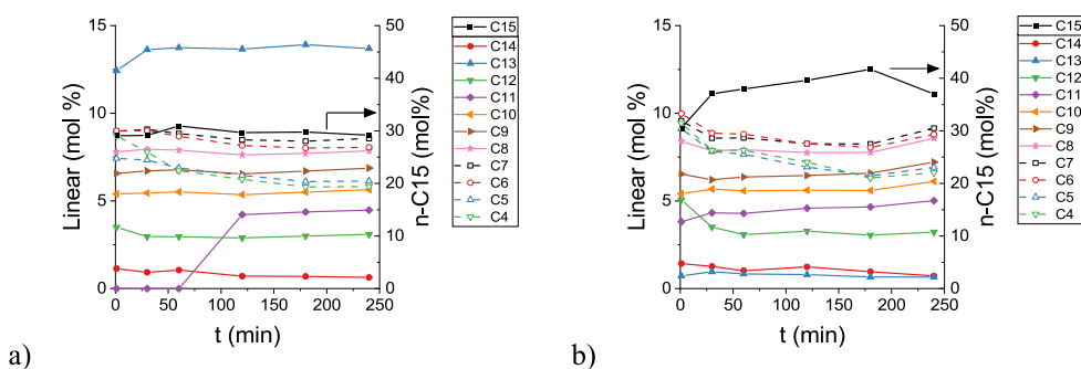
Fig. 7. Linear product distribution (molar fraction) as a function of reaction time in: (a) n-hexadecane hydroisomerization-hydrocracking over Fe 2 Ni 8 catalyst (HXD + cat) and (b) co-processing of isoeugenol hydrodeoxygenation and n-hexadecane hydroisomerization-hydrocracking over Fe 2 Ni 8 catalyst (HXD + IE + cat). Conditions: 573 K and 3 MPa of hydrogen with 100 mL of the reaction volume, 0.1 g of catalyst.
