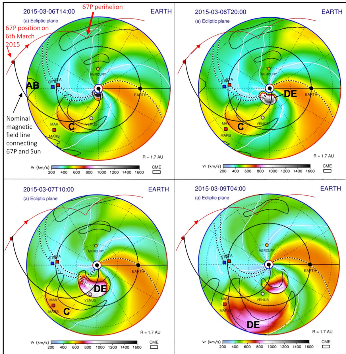
Figure 8. ENLIL simulations of the inner Solar System Part 2: 6–9 March 2015. The Sun is in the center and the color scale indicates simulated solar wind velocities. Date and time are shown in the top left corner of each panel, in UT. The STEREO spacecraft (STA and STB) are shown, as well as major interplanetary coronal mass ejections (ICMEs) (structures surrounded by black solid curved lines). Parker Spiral magnetic field lines that connected the Sun and the STEREO spacecraft, and the Sun and Earth, are shown as black and white lines. The added red line indicates the trajectory of comet 67P, including its perihelion position, its position on 6 March 2015 and the direction toward perihelion. An additional magnetic field line has been added (spiral black solid line) to demonstrate a nominal Parker Spiral field line crossing the location of the comet. Some ICMEs relevant to this study are marked using capital letters; their characteristics are summarized in Table 2.
