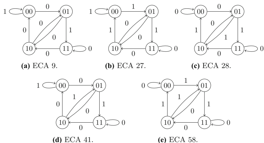
Fig. 1 De Bruijn graphs of the non-regular ECA
