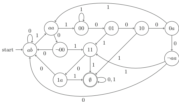
Fig. 2 DFA for orphans of ECA 9. For conciseness we use the binary variables a, b to express arbitrary bits, e.g. aa represents the state \{00, 11\} . By \neg we denote complement, e.g. \neg aa represents \{01, 10\}
