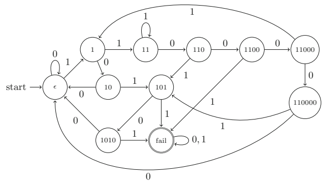
Fig. 3 The DFA from Fig. 2 with states renamed with the suffix they are tracking
