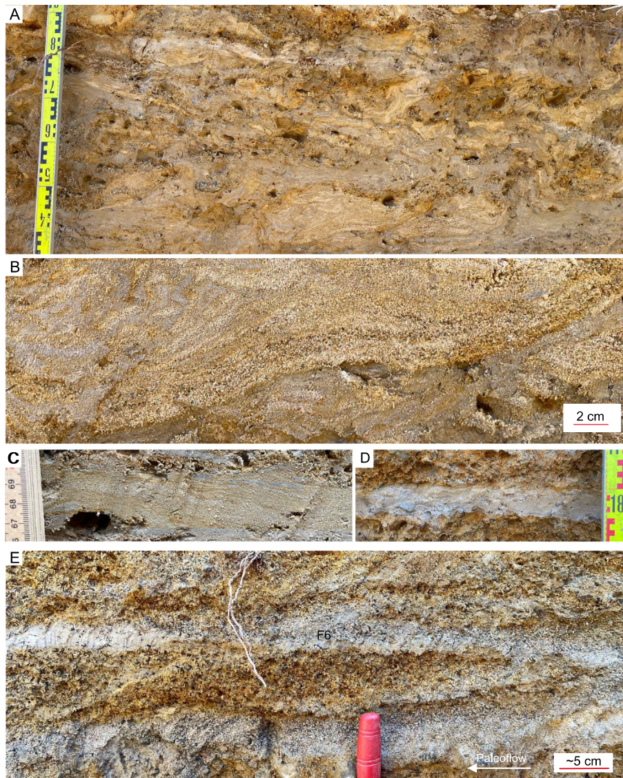
Fig. 5. Facies examples of Sub-unit C1. A) Deformed silt-sand heteroliths showing loading and slumping toward the northern lateral margin of the murtoo (F1). View toward the West. B) Example of sinusoidal stratification overlain by deformed silt-sand couplets. C) Ripple-scale climbing bedforms with apparent upstream oriented (West) climbing orientation. View toward the south. D) Structureless mud bed with pebbels. View toward the south. E) Lenticular sandy gravel. View toward the south.
