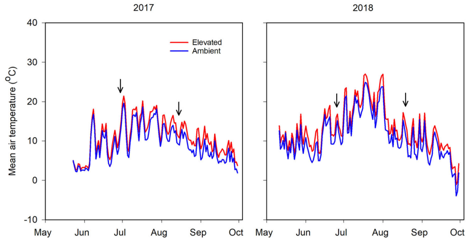
Figure 1. Mean daily air temperatures (°C) for the ambient and heated treatment plots ( n = 3 ) during the May–September growing season in 2017 and 2018 in the open-field experiment at the Turku University Kevo Subarctic Research Station in Utsjoki, Finland. The arrows point at the BVOC sampling dates.
