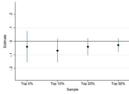
(a) Finnish
