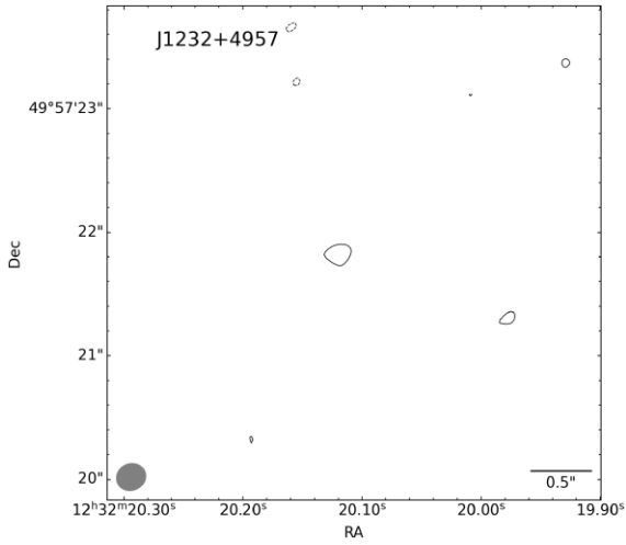
Figure B6. JVL A X-band radio map of J1232+4957, rms = 7\mu\text{Jy beam}^{-1} , contour levels at -3, 3 rms, and beam size 0.98\text{ kpc} \times 0.88\text{ kpc} ( 0.240\text{ arcsec} \times 0.215\text{ arcsec} ).
