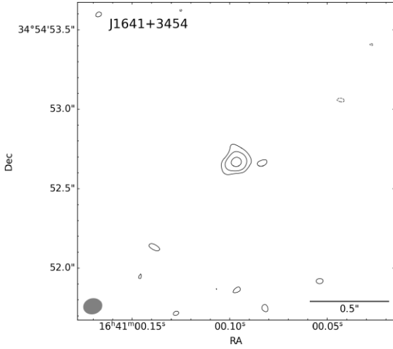
Figure B14. JVLVA K -band radio map of J1641+3454, rms = 8\mu\text{Jy beam}^{-1} , contour levels at -3, 3, 6, 12 rms, and beam size 0.33 \text{ kpc} \times 0.27 \text{ kpc} ( 0.117 \text{ arcsec} \times 0.096 \text{ arcsec} ).
