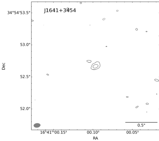
Figure B15. JVLVA Ka -band radio map of J1641+3454, rms = 11\mu\text{Jy beam}^{-1} , contour levels at -3, 3, 6 rms, and beam size 0.29 \text{ kpc} \times 0.18 \text{ kpc} ( 0.103 \text{ arcsec} \times 0.065 \text{ arcsec} ).
