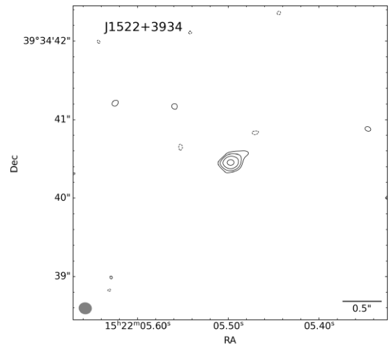
Figure B9. JVL A Ku-band radio map of J1522+3934, rms = 6\mu\text{Jy beam}^{-1} , contour levels at -3, 3, 6, 12, 24 rms, and beam size 0.24\text{ kpc} \times 0.21\text{ kpc} ( 0.162\text{ arcsec} \times 0.142\text{ arcsec} ).
