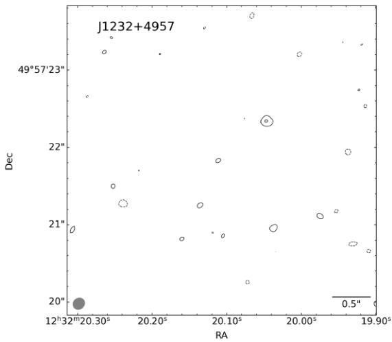
Figure B7. JVL A Ku-band radio map of J1232+4957, rms = 5\mu\text{Jy beam}^{-1} , contour levels at -3, 3, 6 rms, and beam size 0.65\text{ kpc} \times 0.57\text{ kpc} ( 0.159\text{ arcsec} \times 0.141\text{ arcsec} ).
