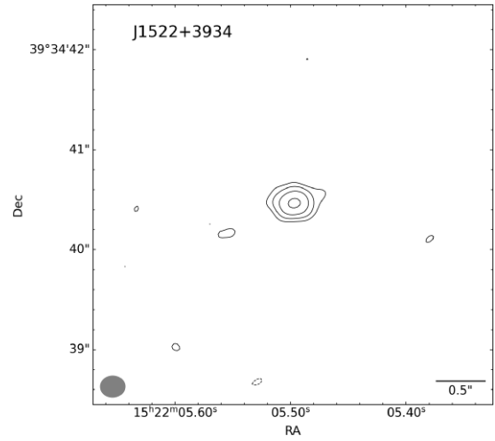
Figure B8. JVL A X-band radio map of J1522+3934, rms = 8\mu\text{Jy beam}^{-1} , contour levels at -3, 3, 6, 12, 24 rms, and beam size 0.36\text{ kpc} \times 0.31\text{ kpc} ( 0.248\text{ arcsec} \times 0.213\text{ arcsec} ).
