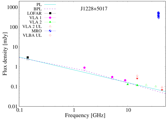
(b) Non-simultaneous radio spectrum of J1228+5017.
