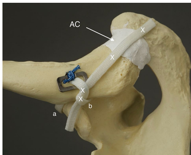
Fig. 2 Model of the right shoulder, posterosuperior view. The reconstructed CC ligament. The anterior limb (a) and the posterior limb (b). The reconstructed AC ligament (AC) and the sites of interrupted No. 2 sutures for fixation and stabilization of the tendon graft (X)
