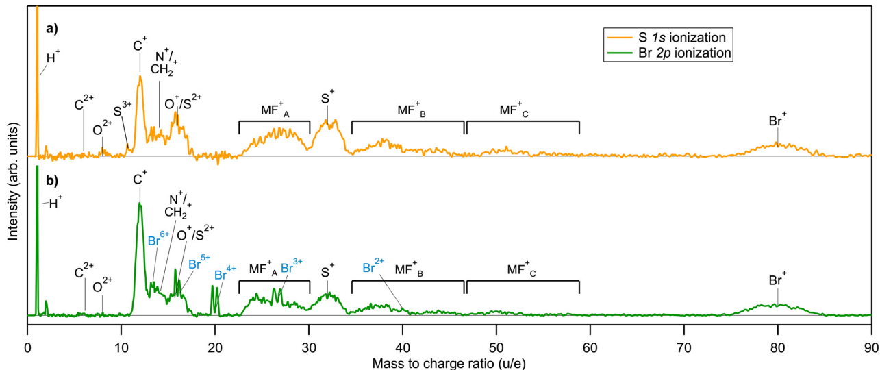
Fig. 4 Ion mass spectra of BrSDU measured in coincidence with the S 1s (a) and Br 2p 3/2 (b) photoelectrons, normalized by the height of the Br + peaks. In addition to the labeled atomic ions, the mass-ranges of significant molecular fragments are marked by MF A,B,C + and CH 2 + . Sharp doublet features Br 3+ –Br 6+ are assigned to contaminant HBr.
