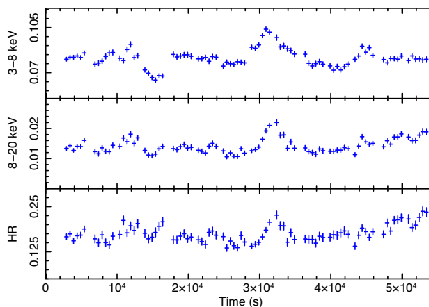
Figure 2. Light curves of Cyg X-2 (in counts \text{s}^{-1} ) in the soft and hard energy band of JEM-X1, and their hardness ratio. Each bin corresponds to 500 s and time is measured from the beginning of the INTEGRAL observation.
