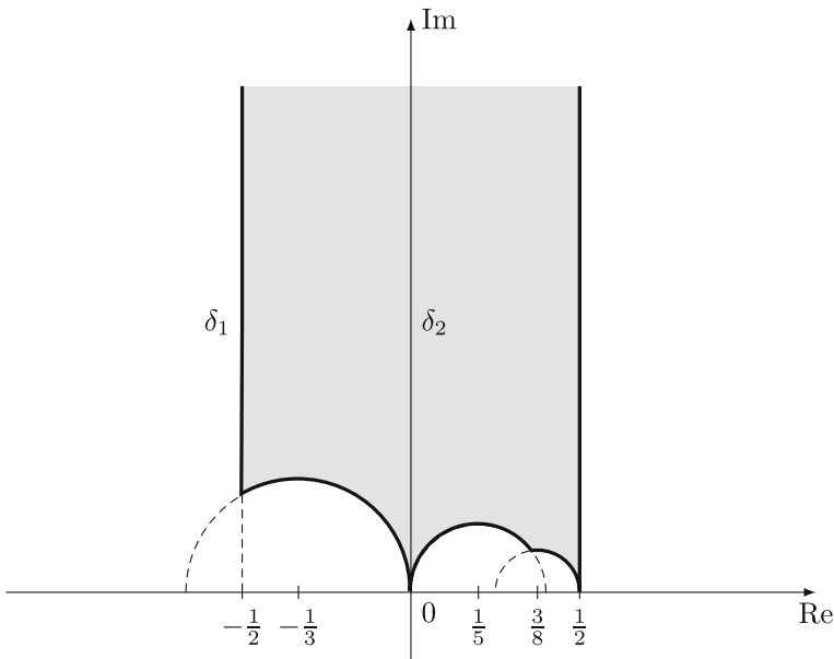
Fig. 1 Fundamental domain for the action of the group \Gamma_0(4) on \mathbb{H}
