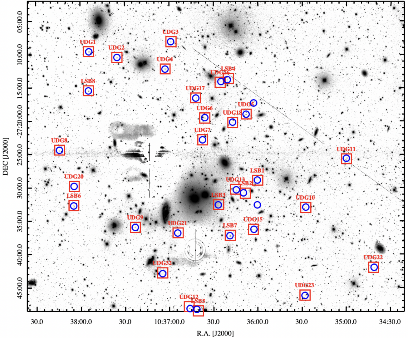
Fig. 2. Optical g -band mosaic from VST of the Hydra I cluster ( 56.7' \times 46.55' \sim 0.8 \times 0.7 Mpc). North is up and East to the left. The two bright stars, close to the cluster core, where modelled and subtracted from the image, as explained in Iodice et al. (2020). The 32 new UDGs and LSB galaxies detected by Iodice et al. (2020) and La Marca et al. (2022a) are marked as blue circles. Red boxes show the LEWIS sample presented in this work and listed in Table 1.
