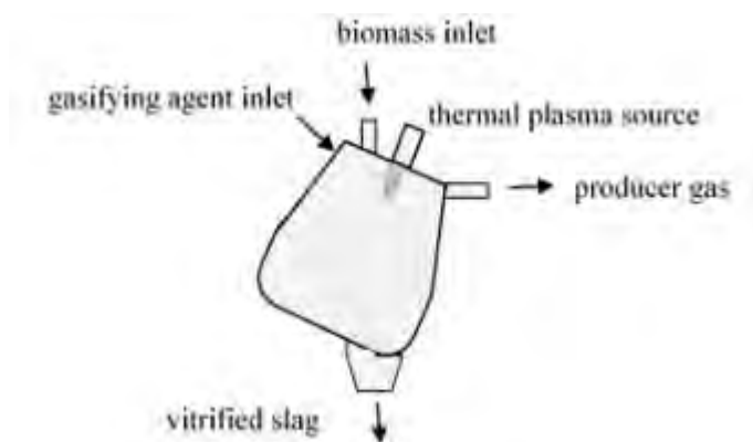
Figure 1. Plasma gasification process reactor.
