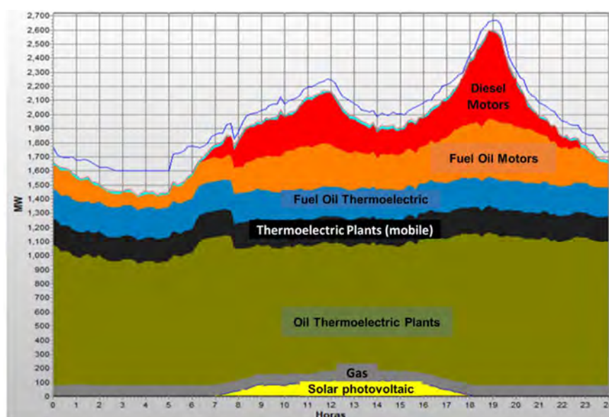
Figure 1b. Load curve January 2021 (Alonso Falcón, Figueredo Reinaldo, and Sifonte Díaz, 2021).
