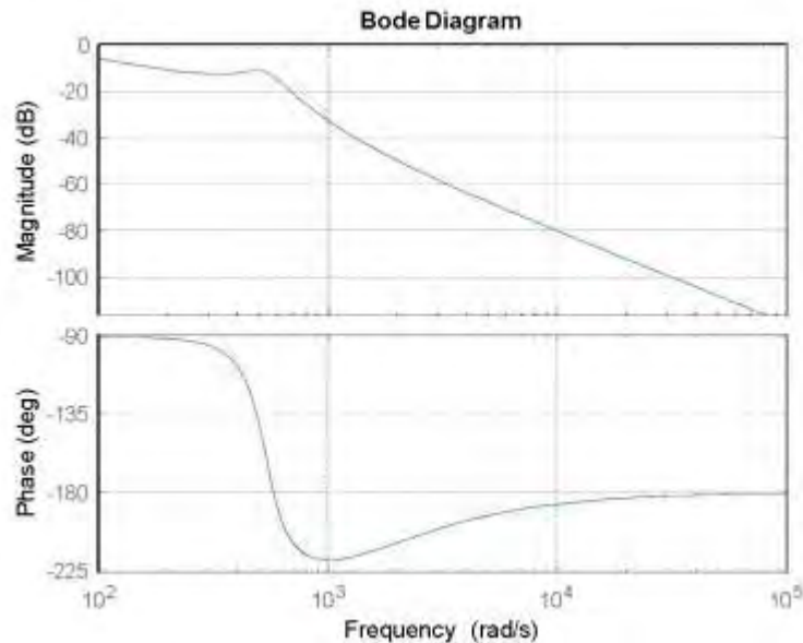
Figure 7. Bode diagram of the LCL filter at the inverter output. For L=10 mH, C=700\mu F , L_g=10 mH and with a value of R_d=1 \Omega .
